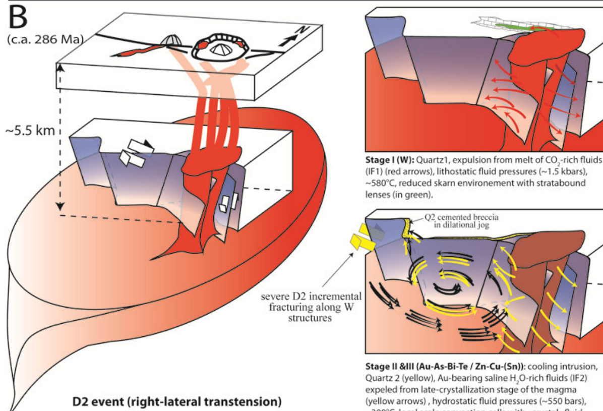
D2 event (right-lateral transtension)
