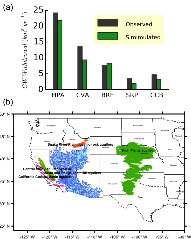
Figure 5. (a) Comparison of simulated total groundwater withdrawals from the selected principal aquifers in the U.S. with the observations. The abbreviations HPA, CVA, BRF, SRP, and CCB denote the High Plains, Central Valley, Basin and Range Basin-fill, Snake River Plain, and California Coastal Basins Aquifers, respectively, which are shown in (b).
