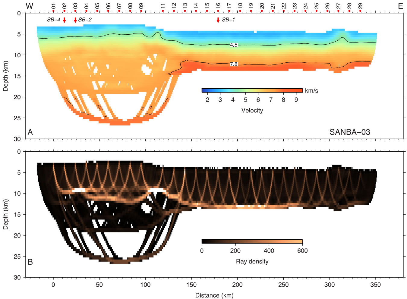
Figure 4. (a) Result of the tomographic inversion of first arrivals on a 0.5 km × 0.5 km grid. The 4.5 and the 7.8 km s -1 iso-velocity contours are trace to give a rough estimate of basement and Moho depth along the profile. OBS locations are indicated by red circles. The 4.5 and 7.8 km s -1 isocontours representing the basement and the Moho are contoured. (b) Ray density of the final tomographic model (0.5 km × 0.5 km).
