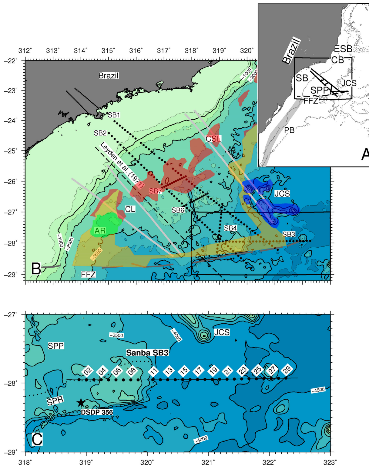
Figure 1. (a) Regional bathymetry map. SB, Santos Basin; FFZ, Florianopolis fracture zone; PB, Pelotas Basin; CB, Campos Basin; ESB, Espiritito Santo Basin; JCS, Jean Charcot Seamounts; AR, Abimaël Ridge; CSL, Cruzeiro do Sul Lineament; CL, Capricornio Lineament; SPP, Sao Paulo Plateau; SPR, Sao Paulo Ridge. Frame shows extension of zoom (b) and grey polygon marks the extension of seaward dipping reflectors in the Pelotas Basin (Blaich et al. 2011; Hinz et al. 1999). (b) Bathymetry of the Santos Basin and location of the wide-angle seismic profiles of the SANBA experiment. Black circles mark seafloor instrument positions, dashed line the deep seismic profile BB' of Leyden et al. (1971), yellow polygons position of the serpentinized upper mantle as proposed by Zalan et al. (2011), orange polygons position of the failed spreading centre as proposed by Meisling et al. (2001), green polygon Abimaël Ridge and blue polygon position of the Jean Charcot Seamounts. Outlined box marks the position of the zoom (c) Bathymetry of the research area along profile Sanba 3. Black circles mark OBS positions and black line the shot positions. Position of DSDP drill hole 356 is marked by a star. Grey area marks extend of the Sao Paule Ridge from Kumar & Gamboa (1979).
