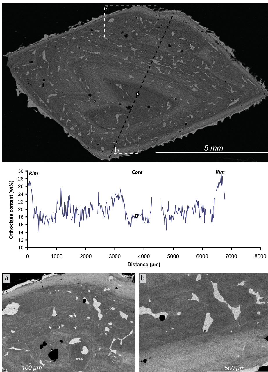
Fig. 1. Upper panel: Potassium X-ray maps of a sectioned anorthoclase crystal (sample eb05027a2 ) showing remarkable oscillatory zoning. Irregularly-shaped melt inclusions are clearly visible as brighter (K-rich) areas. Central panel: EMP transect reported in terms of orthoclase end member content (in %). The location of the transect is shown on the X-ray map; the white circles show corresponding points between the analysis and the crystal. The starting point of the transect is the upper right portion of the crystal. Gaps in the transect indicate the presence of melt inclusions. Lower panel: left hand side: Close-up potassium X-ray maps of area (a), the location of which is shown on upper panel map. Notice the patchiness of the central zones (labelled ptch ) and the embayed zone boundaries (labelled emb ), both textures indicative of out of equilibrium, resorption events. Right hand side: Close-up potassium X-ray maps of area (b), the location of which is shown on upper panel map. This map shows the strong contrast between the last two zones closest to the rim of the crystal, the relatively straight boundary and gradual change of composition.
