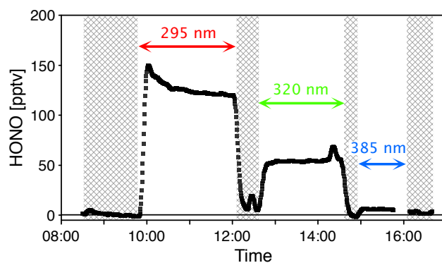
Figure 5. Photochemical release of HONO from a surface snow collected at DC when irradiating it at a temperature of −16 °C (see Table 1) and inserting filters with cut-off points at 295, 320, and 385 nm on the xenon arc lamp (see Sect. 4). Vertical grey bands correspond to periods over which the lamp was switched off.
