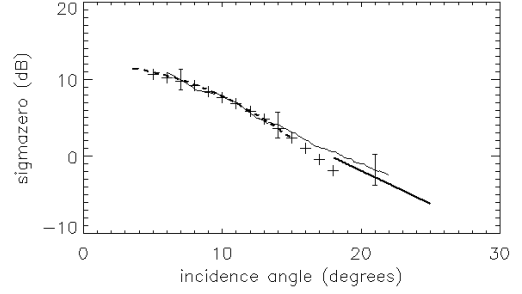
Figure 1: Normalized radar cross-section averaged over the azimuthal directions, as a function of incidence angle. Thin solid line : obtained from KuROS on 6 March 2013 (wind speed is 9m/s and significant wave height is 5.3m); the error bars indicate the standard deviation over an incidence angle bin of 1°. Dashed line : model from [7]. + signs : quadratic fit to TRMM data [8]. Thick solid line : NSCAT empirical model [9].
