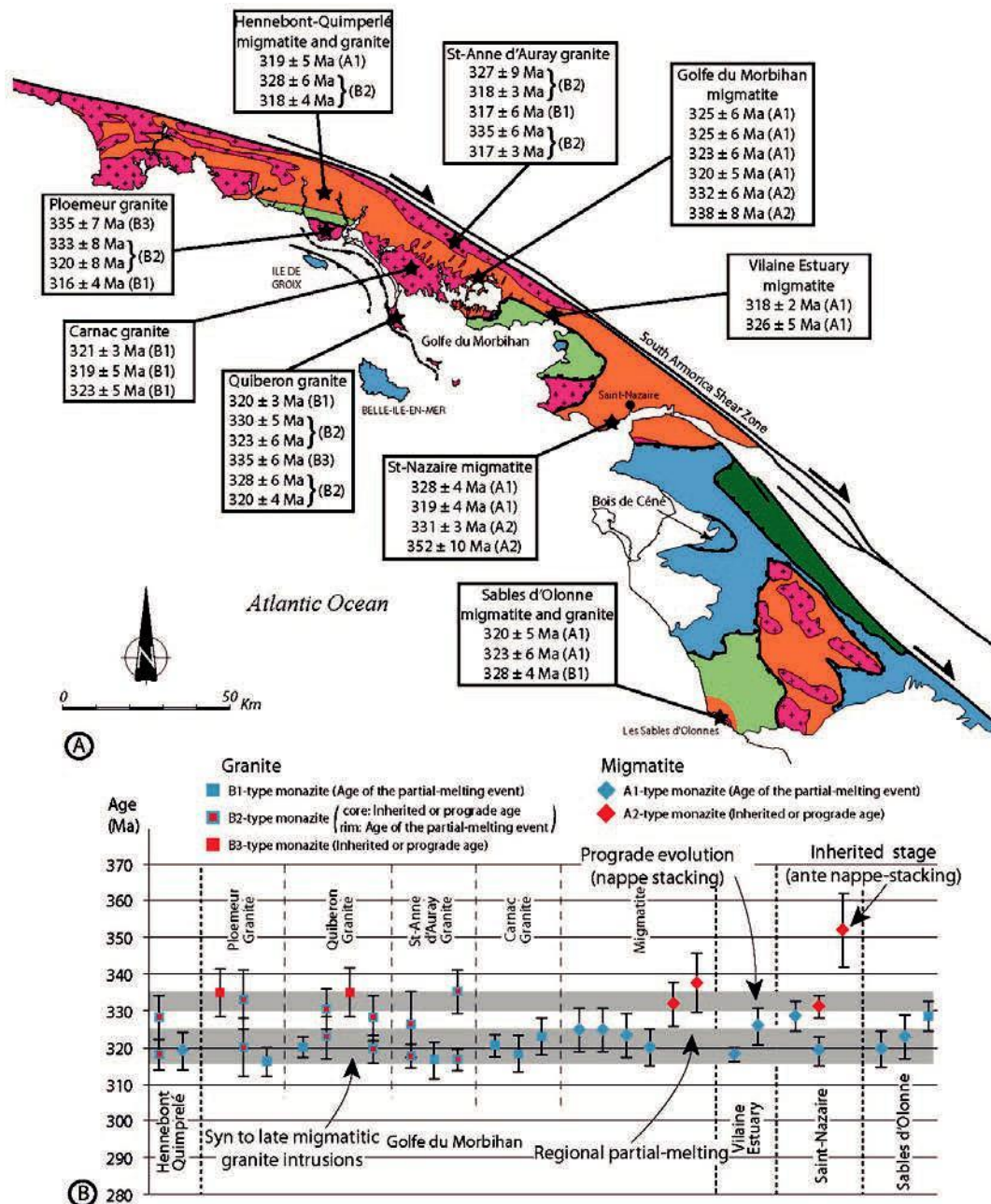
FIG. 11. – Synoptic chart of the U-Th/Pb geochronological results across the coastal South Armorican domain. Despite local partial age overlapping, 3 different stages can be distinguished. Old inherited ages remain rare (e.g. the 352 Ma age), whereas a pre-anatectic, prograde episode probably associated to nappe-stacking is recorded throughout the study area at ca. 335-330 Ma. Partial-melting that probably starts at ca. 325 Ma, and became widespread during the 325-320 Ma period, accompanied by the accumulation of large volume of anatectic melts as anatectic granites (e.g. Sainte-Anne d'Auray granite). The ca. 320-318 Ma age is ascribed to late or even post-migmatitic granites (e.g. Carnac, Ploemeur and Quiberon granites).
