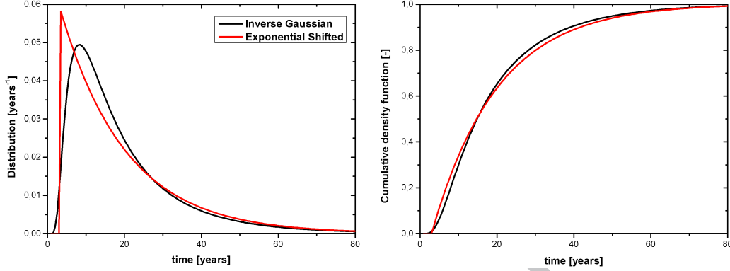
Figure 14: Distribution and cumulative density function associated of an Inverse Gaussian distribution with (\mu, \lambda) = (20, 30) years and of the Shifted Exponential distribution that fits the observables C_{CFC}^{IG} and C_{Kr}^{IG} obtained with the Inverse Gaussian distribution.
