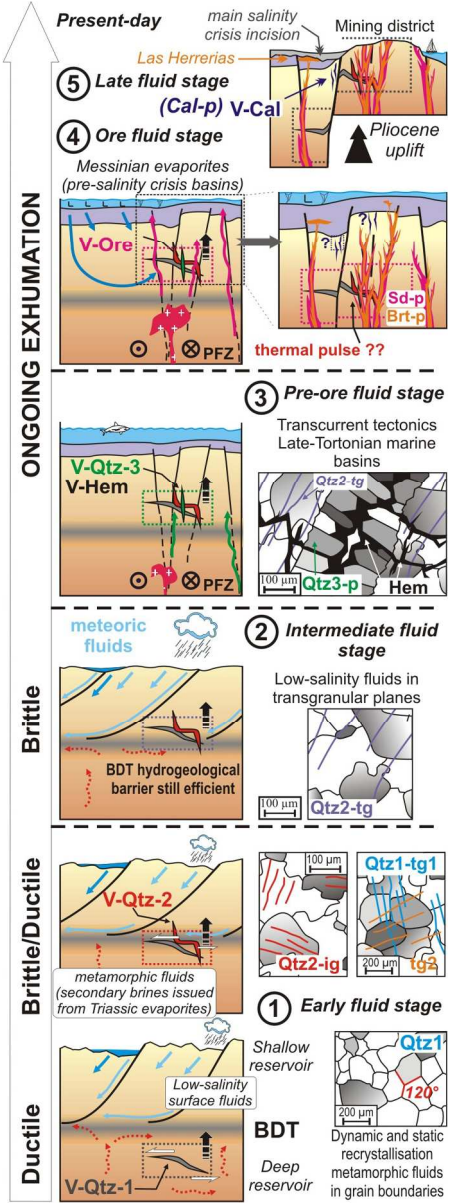
Exhumation of the Sierra Almagrera with associated tectonic regime, paleo-orographic evolution and paleofluid sequence 77x208mm (300 x 300 DPI)
