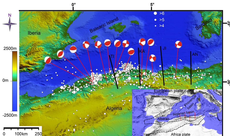
Figure 1. Topography, bathymetry by ETOPO1 1-min global relief ( www.ngdc.noaa.gov ) and seismicity of the Algerian margin (epicentres and focal mechanisms). Solid lines indicate the location of the SPIRAL wide-angle profiles. Inset shows a more regional tectonic sketch of the Mediterranean Region (modified after Barrier et al. 2004).
