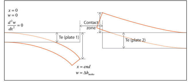
Figure 3. Setup of the flexural models. Te is the effective elastic thickness in km. The deflection ( w ) is set to zero at the extremities of the plates, and imposed at the plate junction.
