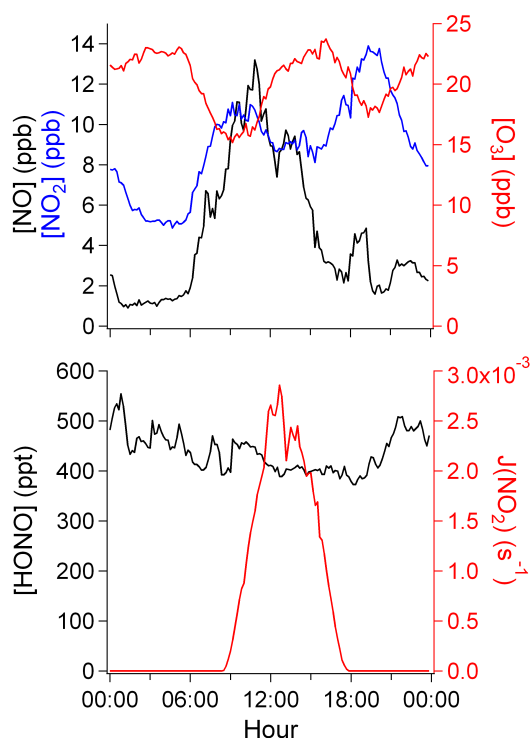
Fig. 4. Average diurnal 10 min profiles for \text{O}_3 , \text{NO}_x , HONO, and J(\text{NO}_2) during the MEGAPOLI winter campaign (local time).
