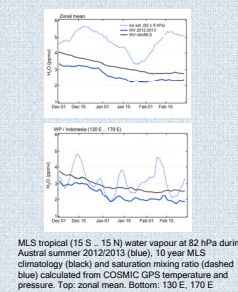
Captions in the plot indicate the approximate latitudinal location and time period of the measurement campaigns
