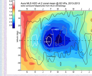
Captions in the plot indicate the approximate latitudinal location and time period of the measurement campaigns
