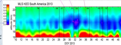
Bottom: Water vapor profiles (FLASH-B and Pico-SDLA) above Bauru and climatological profile from MLS for the given time period. Top: MLS H 2 O time series above tropical South America, vertical lines = balloon soundings.
