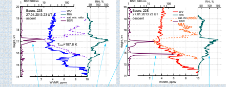
Vertical profiles of water vapour (FLASH-B), backscatter ratio (COBALD), RHice and saturation mixing ratio (PT from Vaisala RS92) obtained during balloon ascent (left) and descent (right).
