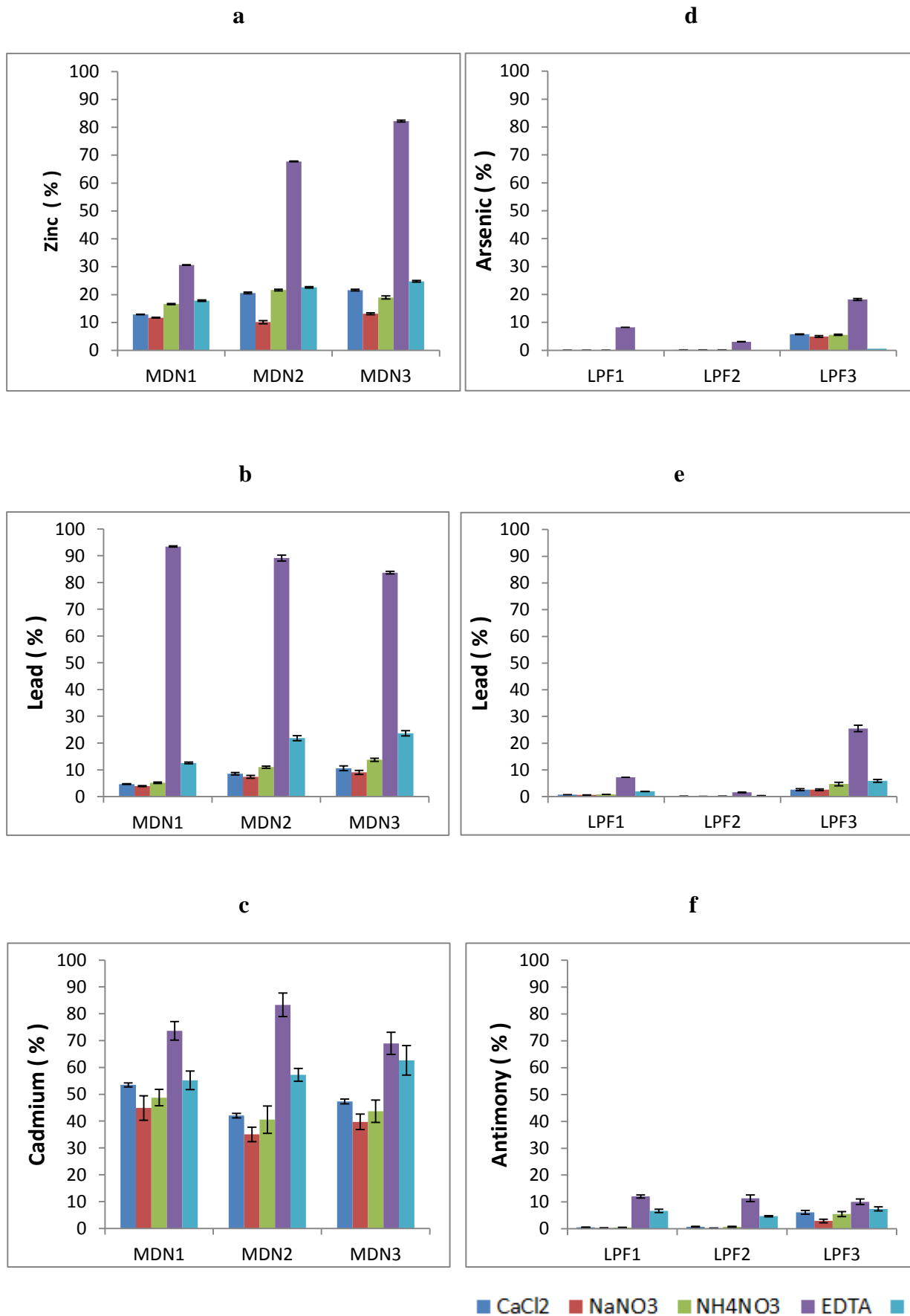
Fig. 1 Extractable potentially toxic elements (Zn, Cd, Pb, As and Sb) (%) by various single extractants (CaCl 2 , NaNO 3 , NH 4 NO 3 , EDTA and DTPA) for MDN site (a, b and c) and LPF site (d, e and f).
