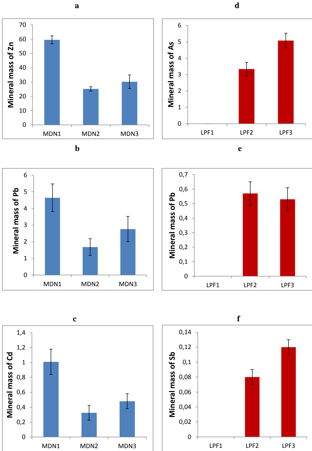
Figure 2 Mineral masses of Zn, Pb, Cd, As and Sb (mg/plant) in the dwarf bean primary leaves for MDN site (a, b and c) and LPF* site (d, e and f).
