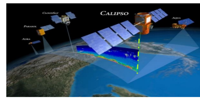
Fig1: CALIPSO's lidar track
