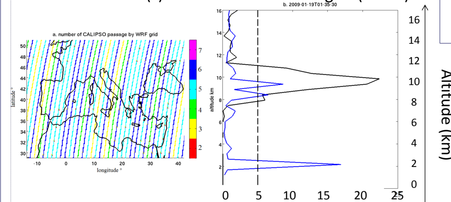
Fig2: (a) CALIPSO track occurrence in JJA 2008 (b) example of two SR GOCCP profiles (19/01/2009 at night)
