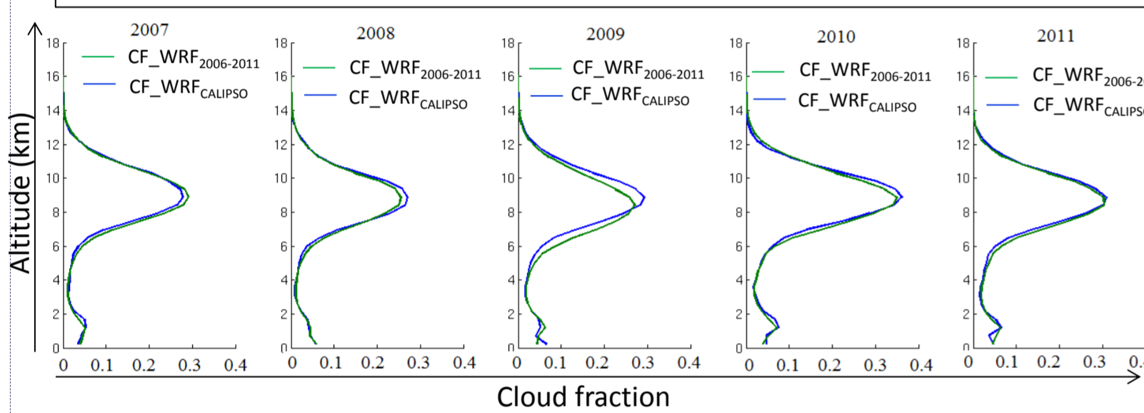
Fig4: horizontally averaged cloud fraction monthly means in WRF sampling (blue) and in CALIPSO sampling from 2007 to 2011
