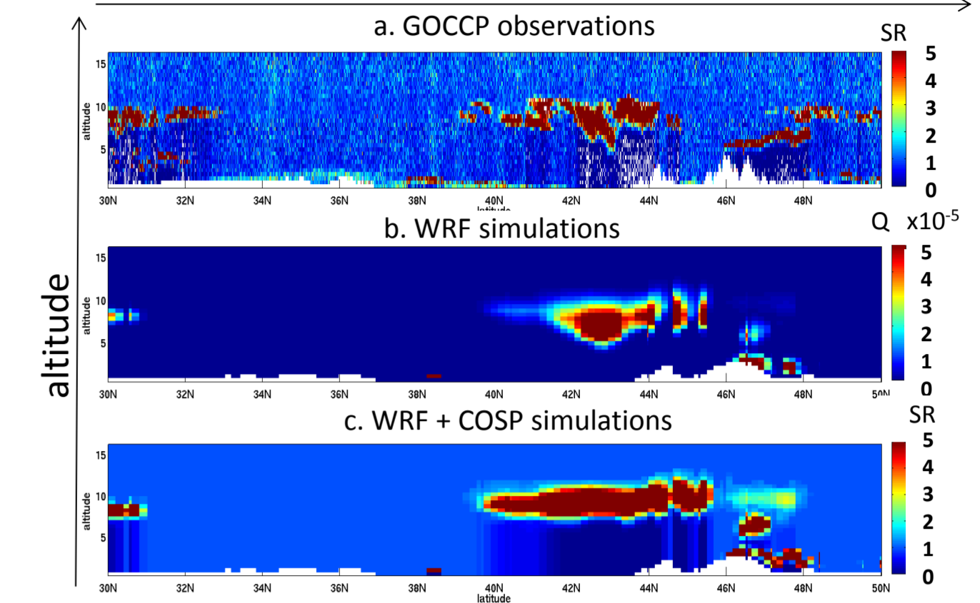
Fig3: Instant SR 19/01/2009 night: (a) Observations, (b) WRF simulations and (c) WRF+lidar simulator simulations
