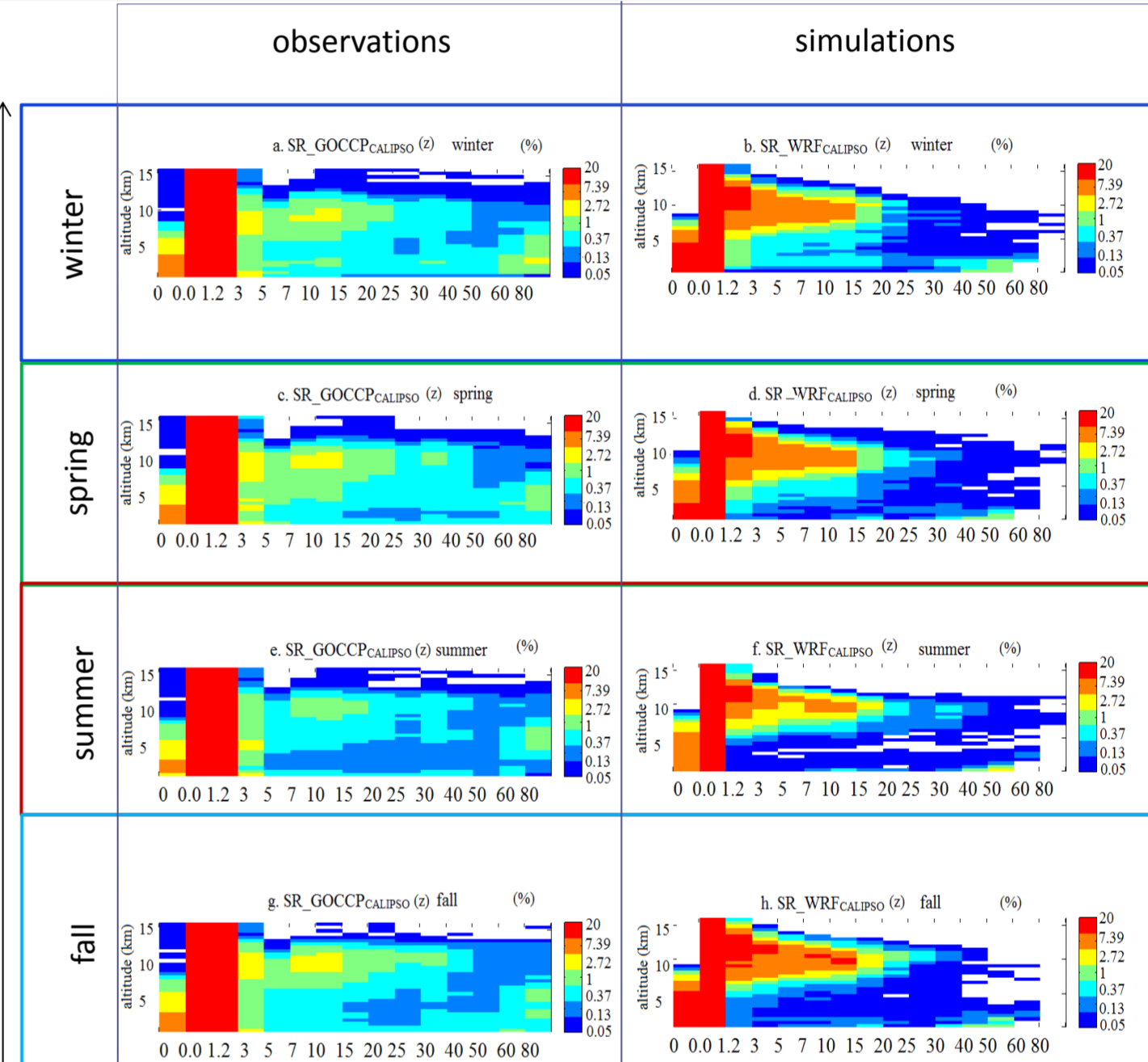
Fig7: SR histograms for cumulated SR between 06/2006 and 11/2011 in winter, spring, summer and fall for observations and simulations
