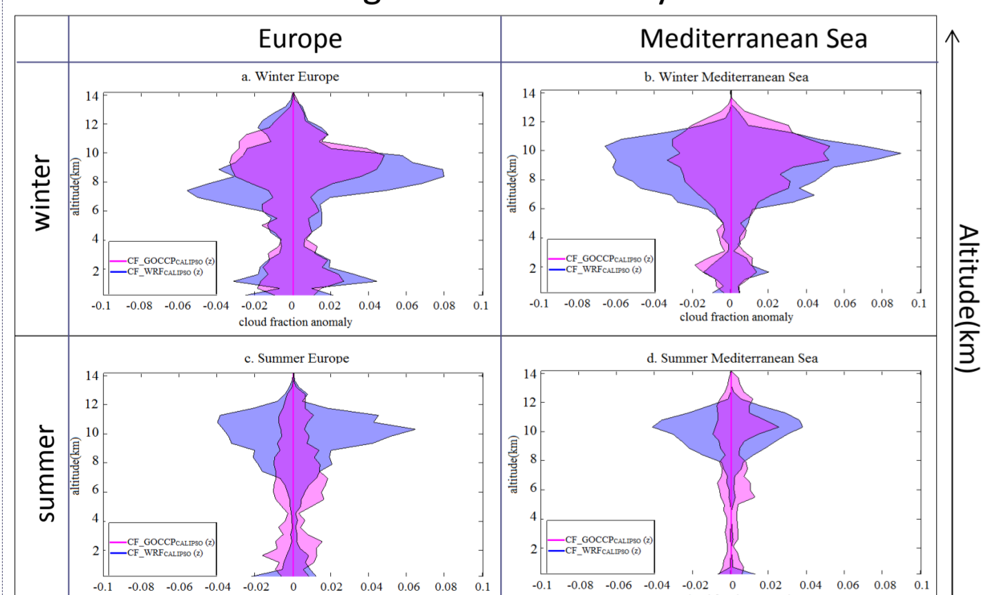
Fig8: Enveloppe of inter annual CF anomaly compared to mean 2006-2011 of horizontally averaged CF (observations; simulations with CALIPSO-sampling) for Europe and Mediterranean Sea in summer and winter
