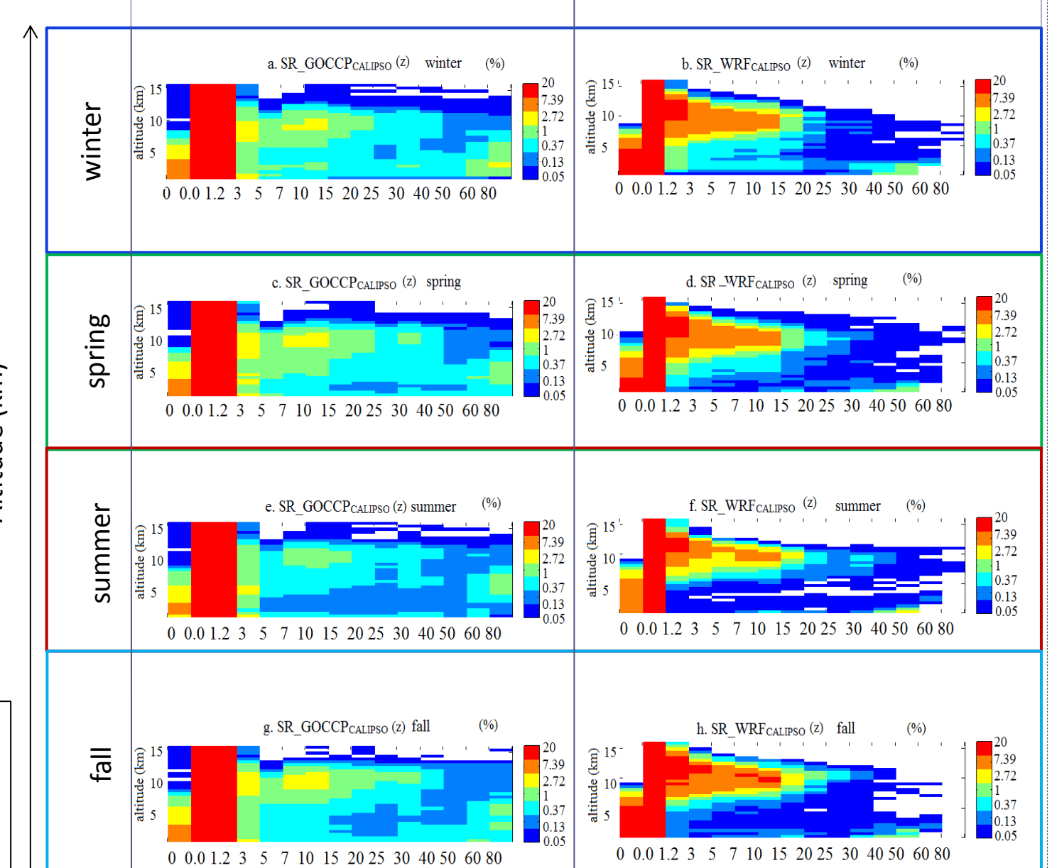
Fig7: SR histograms for cumulated SR between 06/2006 and 11/2011 in winter, spring, summer and fall for observations and simulations
