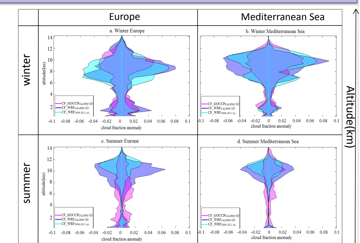
Fig10: Envelope of inter annual CF anomaly compared to mean 2006-2011 of horizontally averaged over Europe (only continent) and over the Mediterranean sea (only sea) cloud fraction (observations; simulations with sat. sampling; simulations with WRF sampling) for winter and summer
