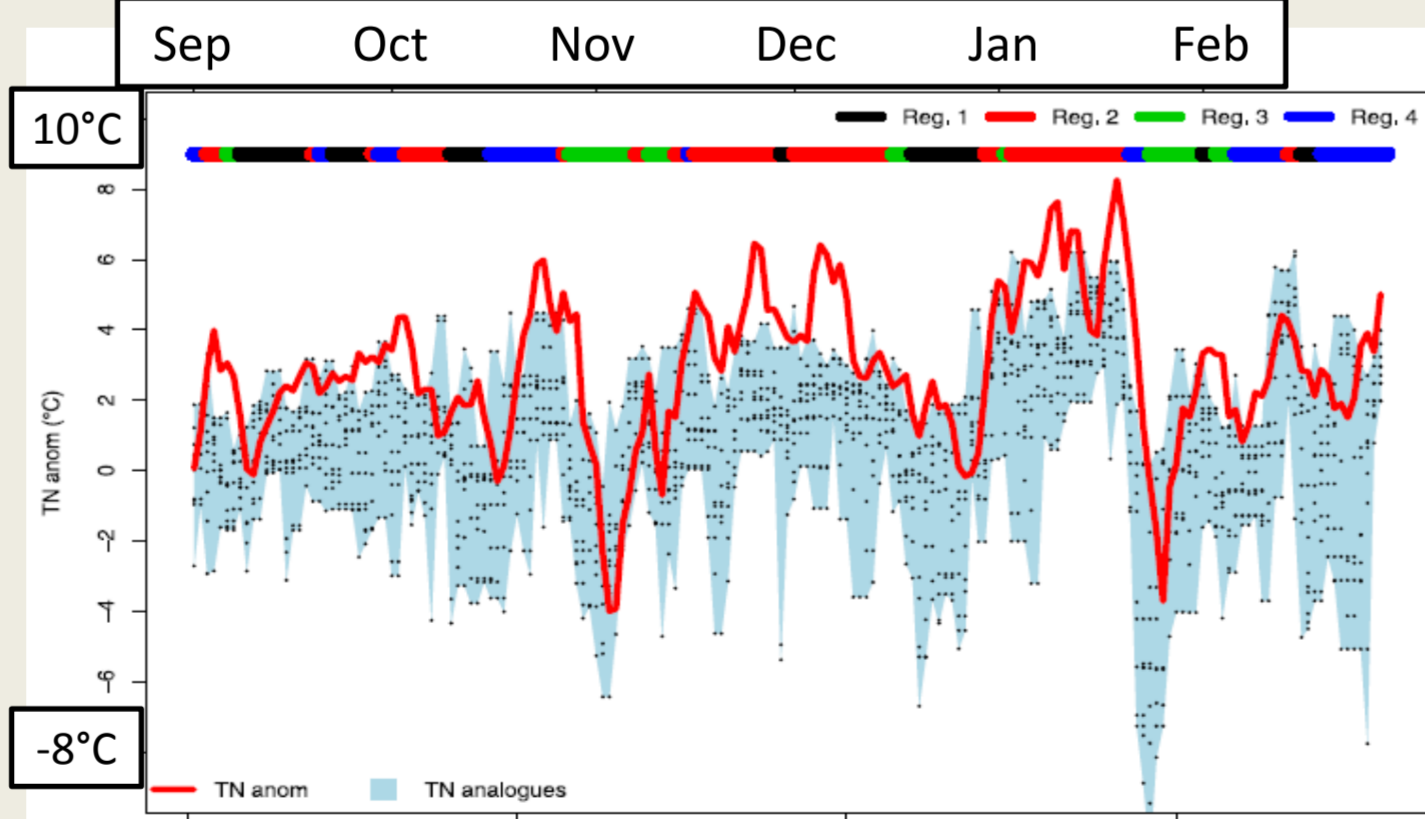
Fig10: time evolution of the daily minimal temperature anomaly with 10 best circulation analogues (dots) and their range (blue shade) (You et al. 2007)
