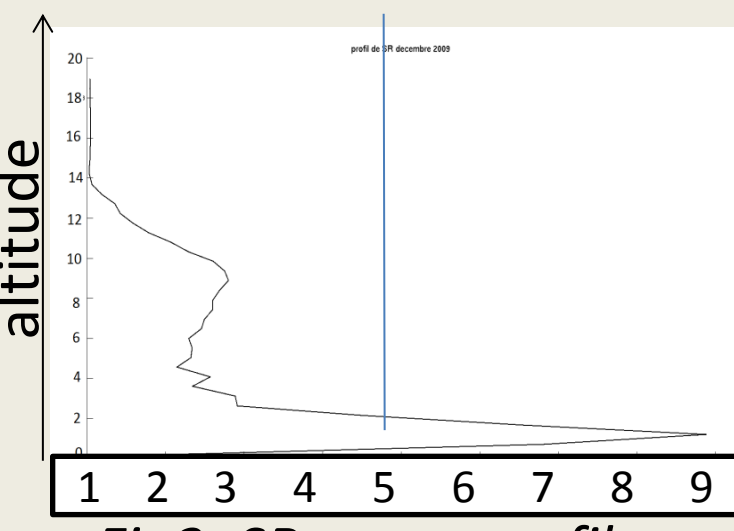
Fig2: SR mean profile 12/2009
