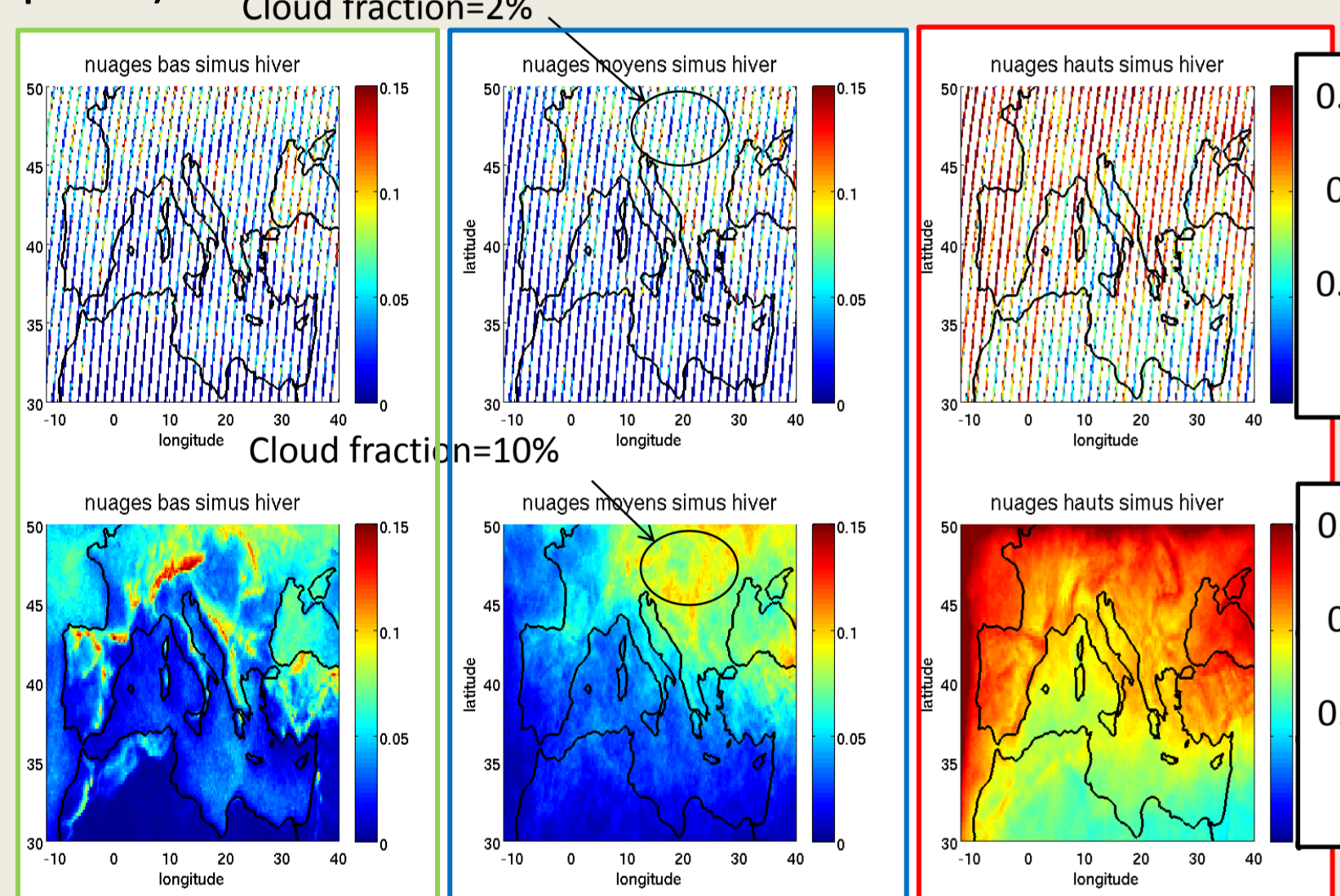
Fig5: low, mid and high simulated clouds with CALIPSO sampling on the top and WRF sampling on the bottom
