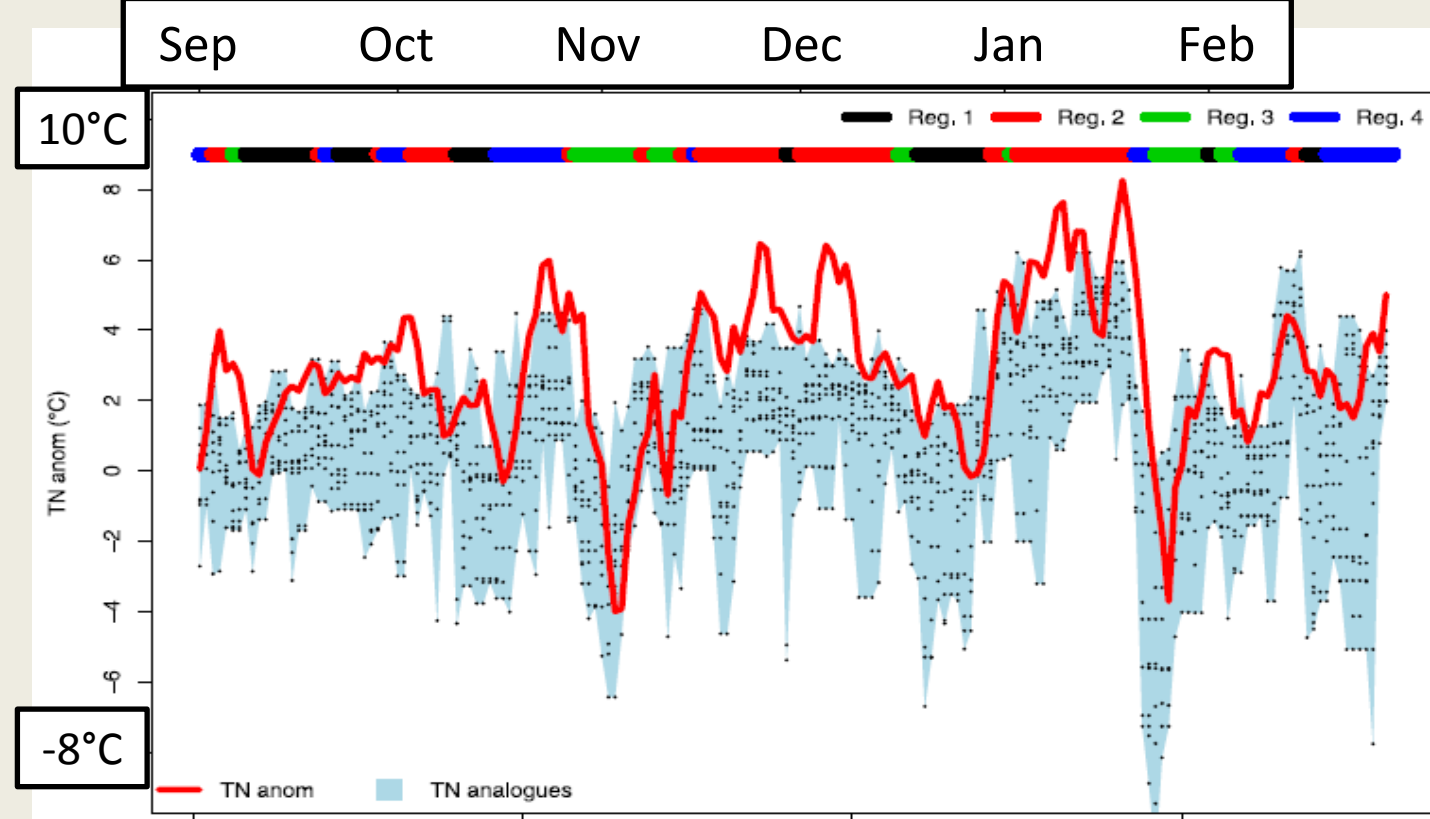
Fig10: time evolution of the daily minimal temperature anomaly with 10 best circulation analogues (dots) and their range (blue shade) (Yiou et al. 2007)
