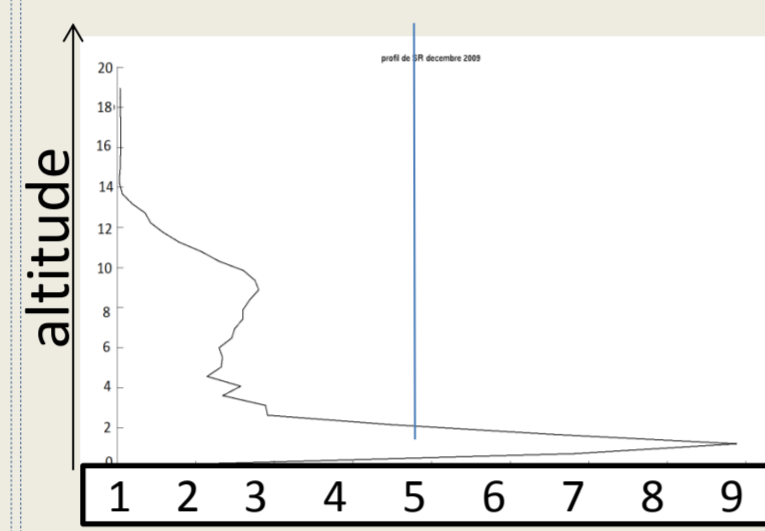
Fig2: SR mean profile 12/2009
