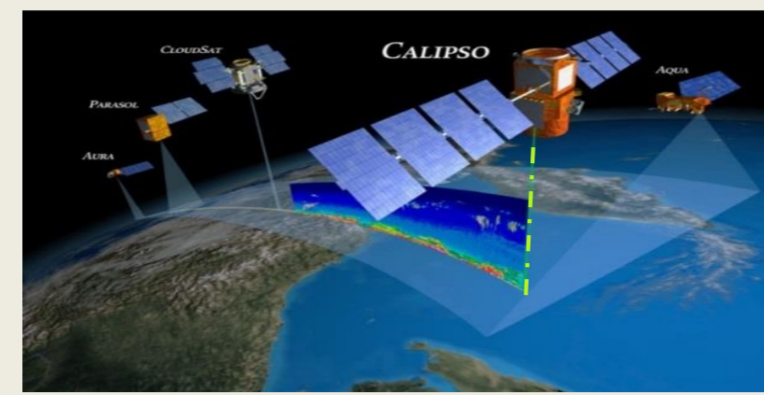
Fig1: CALIPSO's lidar track
