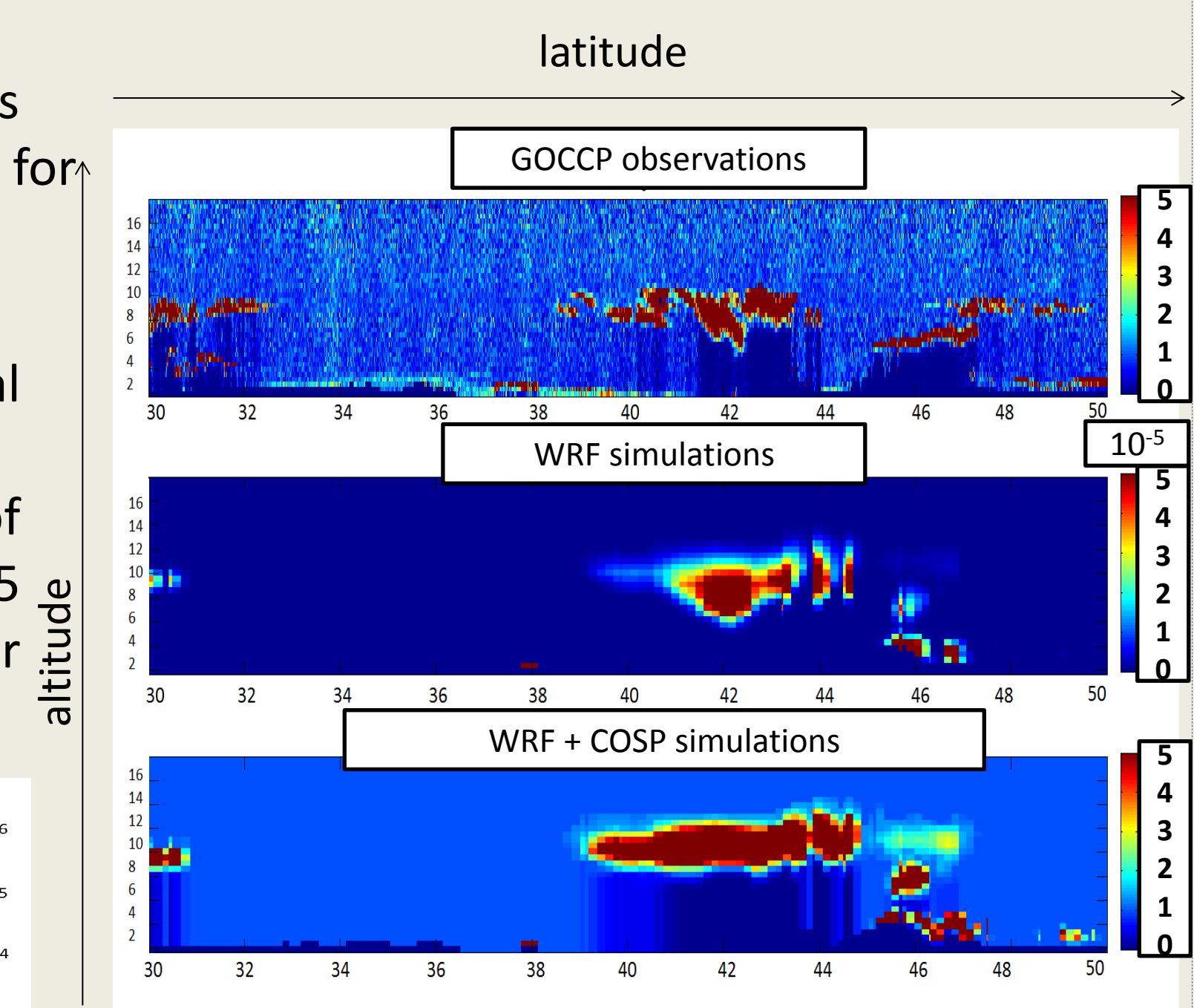
Fig4: Instant SR 2009 01 19 night: Observations, WRF simulations and WRF+lidar simulator simulations
