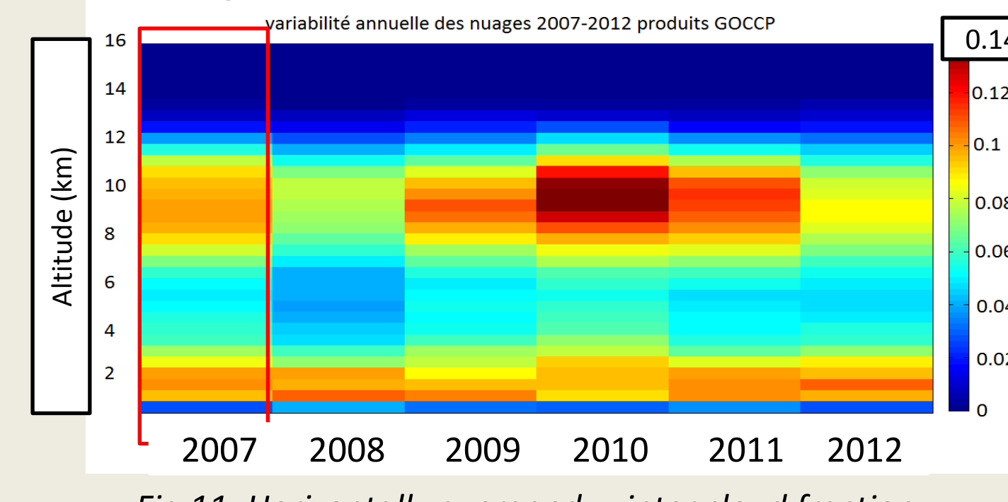
Fig 11: Horizontally averaged winter cloud fraction annual evolution
