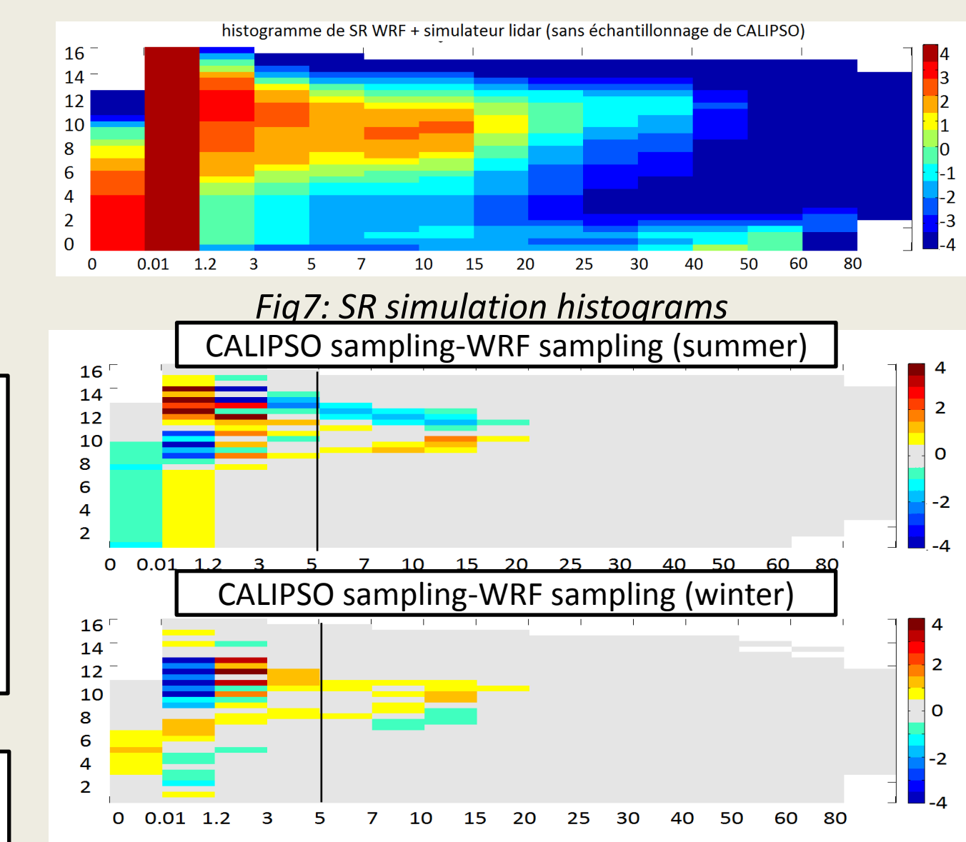
Fig6: Difference between SR simulated histograms CALIPSO sampling - WRF sampling in summer (top) and winter (bottom)
