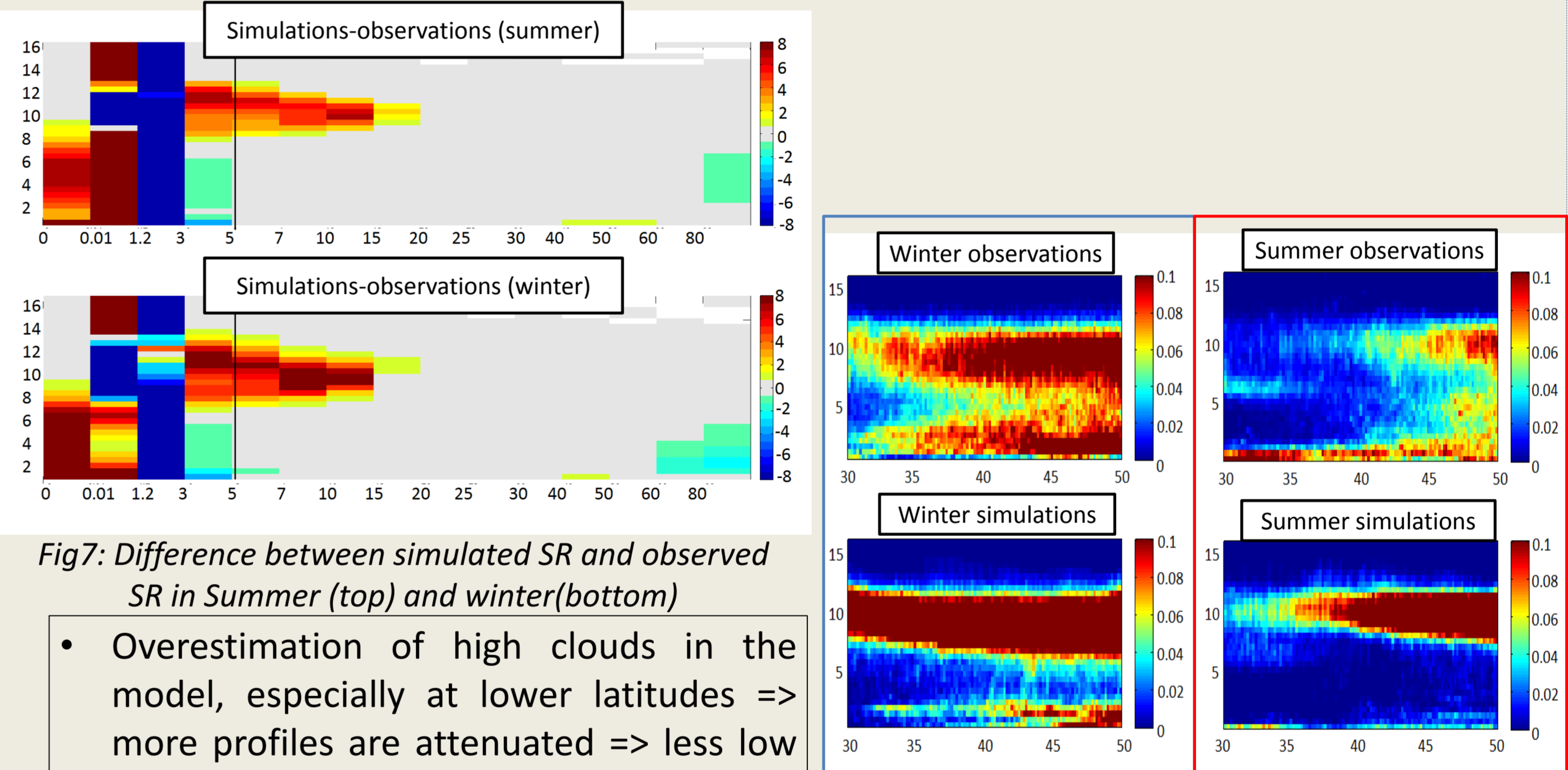
Fig 8: Vertical clouds distribution zonally averaged for observations (top) and simulations (bottom) in summer and winter
