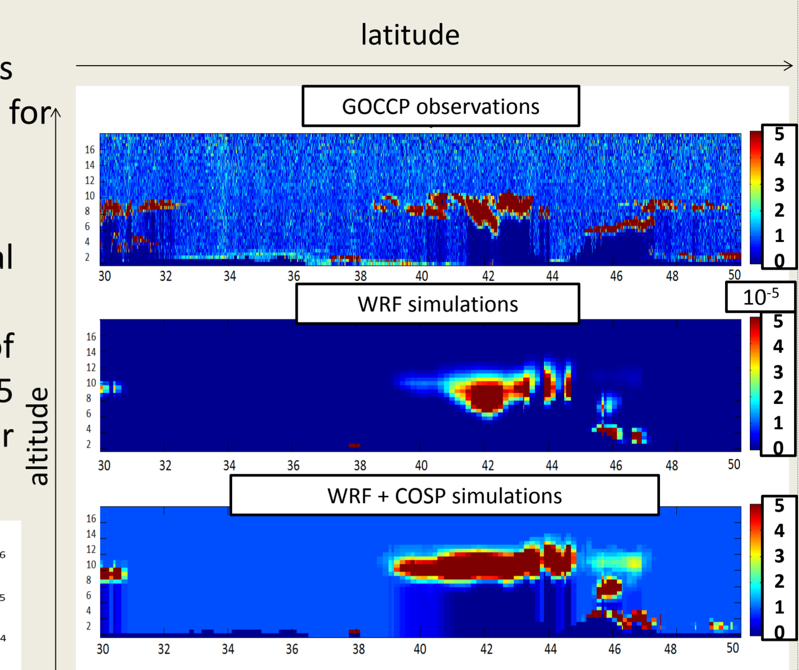
Fig4: Instant SR 2009 01 19 night: Observations, WRF simulations and WRF+lidar simulator simulations
