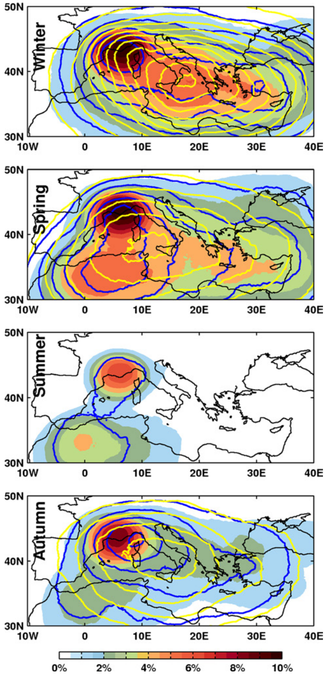
Fig. 6 Seasonal frequency of areas affected by cyclones for SimREF, for cyclones with intensity of 8-10 \times 10^{-5} \text{ s}^{-1} (in color), for cyclones with intensity of 10-12 \times 10^{-5} \text{ s}^{-1} (blue line contours starting from 1 with 1 % of interval) and for cyclones with intensity of more than 12 \times 10^{-5} \text{ s}^{-1} (yellow line contours starting from 1 with 1 % of interval)
