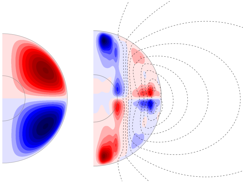
Figure 6: Left: the simple magnetic field used in eq. 9 to model the magnetic pumping. Right: axisymmetric part of the growing magnetic field for Rm = 1000 and \Lambda = 0.9 . The colormap shows the azimuthal (toroidal) component and the black contours show the meridional (poloidal) field lines. The small gray circle marks the size of Earth’s inner-core, although we have none in our study.
