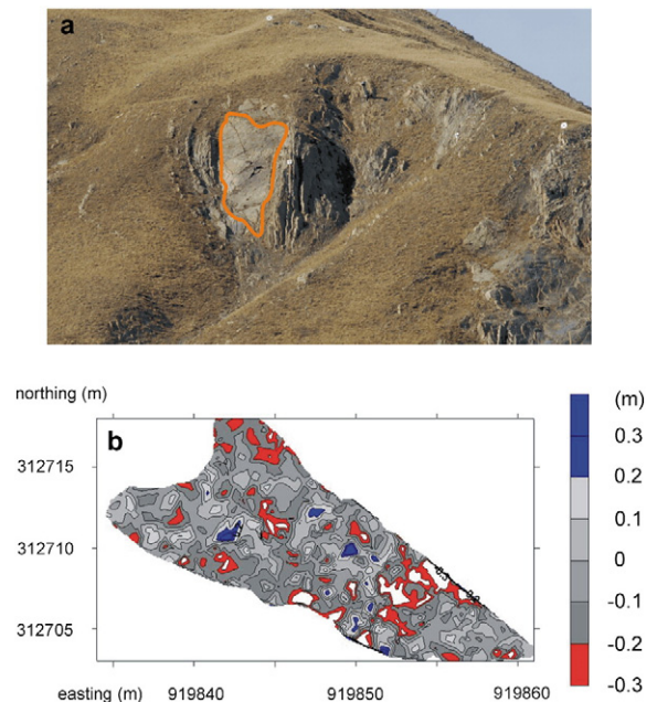
Fig. 9. Comparison between digital elevation models from photogrammetry and laser scanning on a test area. Top: rocky area on the top of path no. 2 use to compare elevation models. Bottom: differences in elevation models: no systematic bias is detected (the average elevation difference is 0) and the standard deviation is 0.11 m.
