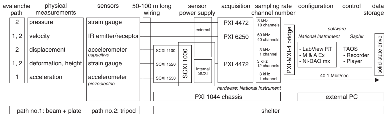
Fig. 3. Schematic of measurements and data acquisition performed within the flow for the 2 avalanche paths, from sensors to data storage. Analog-to-digital conversion is performed by PXI-4472 (24 bits) and PXI-6250 (12 bits) modules. Analog signals conditioned by SCXI modules are multiplexed by the SCXI-1000 platform before digital conversion by the PXI-4472.
