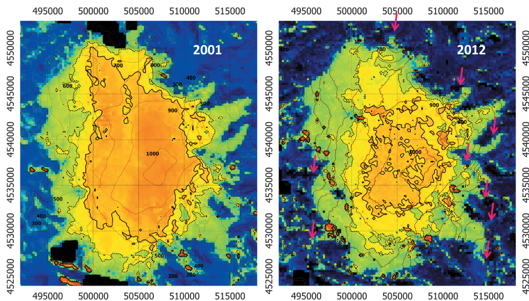
Figure 6. Comparison between albedo maps for (left) 9 March 2001 and (right) 26 April 2012. For key to pixel colors, see Figure 2a. The snow line is represented by black lines (dotted line for the limit between ice and fragmented snow cover and continuous line for the limit between fragmented snow cover and full fresh snow cover), and contour lines in 2000 (SRTM DEM) and 2009 (SPOT DEM) respectively are in burgundy (numbers indicate contour line elevations in m asl). The pink arrows in the 2012 image point to sites where ice tongues or termini disappeared between 2001 and 2012. Coordinates are in UTM (Zone 42S).
