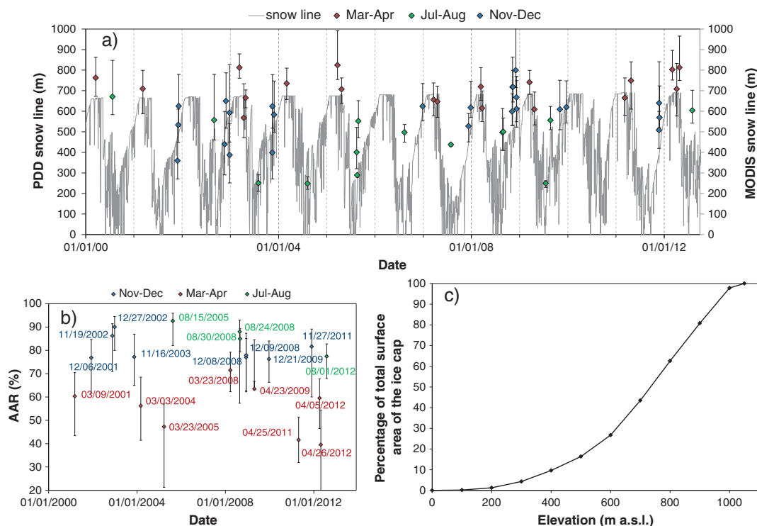
Figure 5. (a) Comparison between Ampere Glacier snow line computed with the PDD model and discrete snow line elevations for the Ampere Glacier obtained from albedo maps derived from MODIS images. Error bars are given for a snow albedo limit between 0.55 and 0.65 on the MODIS images. (b) Changes in the ratio of the accumulation area (snow-covered area) to the surface area of the entire ice cap between January 2000 and August 2012, for three periods: November–December (blue), March–April (red), and July–August (green) derived from clear-sky MODIS images. Error bars are also indicated for a snow albedo limit between 0.55 and 0.65 on the MODIS images. (c) Hypsometry of the Cook Ice Cap in 2009, i.e., the percentage of the surface area of ice cap below a given elevation.
