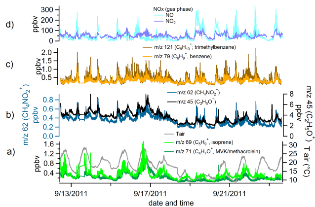
Figure 3. The concentration in ppbv of PTR-MS VOC species-identified isoprene and methyl vinyl ketone/methacrolein (left axis, a ), VOC species associated with diesel exhaust ( \text{CH}_4\text{NO}_2^+ , \text{C}_2\text{H}_5\text{O}^+ , b ), VOC species associated with gasoline exhaust ( \text{C}_6\text{H}_7^+ , \text{C}_9\text{H}_{13}^+ , c ). NO and \text{NO}_2 (gas-phase) ppbv concentrations ( d ) and ambient temperature (right axis, a ) during the measurement period are also shown.
