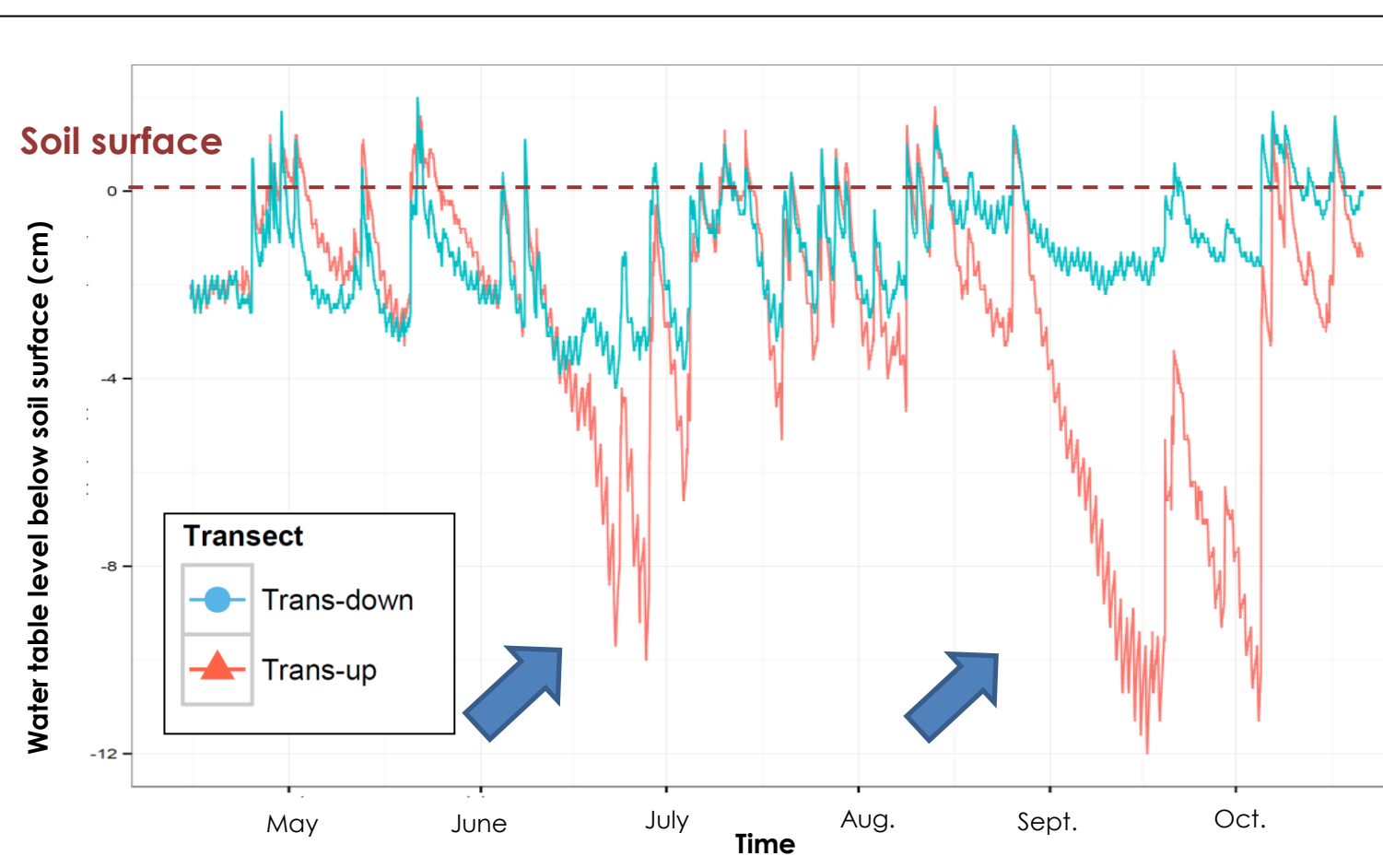
Fig. 2: Fluctuations of water table since restoration
