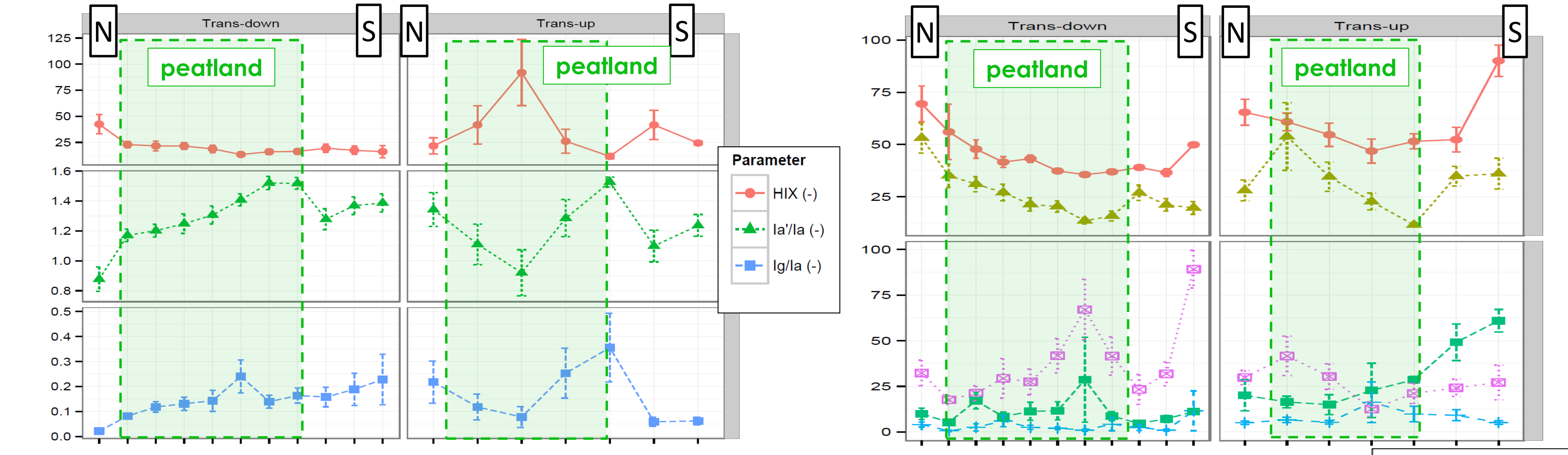
Fig. 9: Spatial variations of peatwater geochemistry
