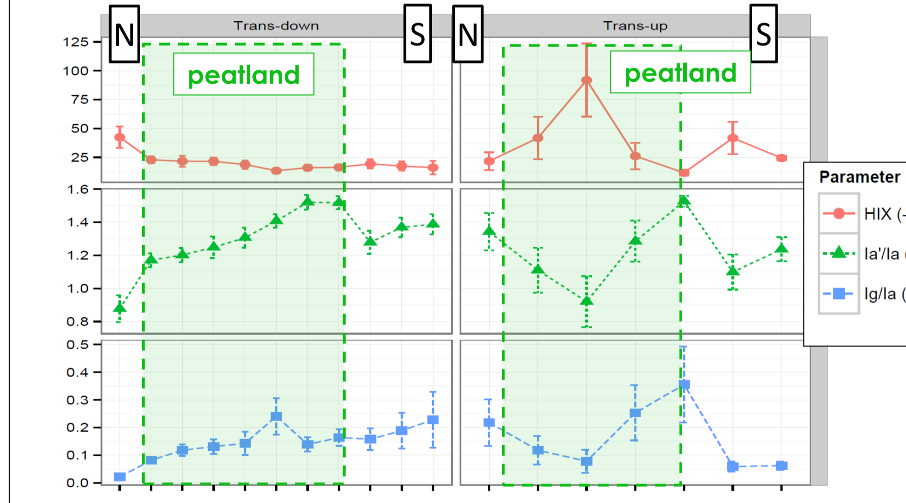
Fig. 8: Spatial variations in 3D fluorescence of DOM
