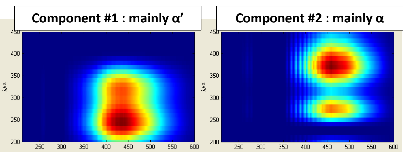
Fig. 4: Example of EEM from La Guette peat water
