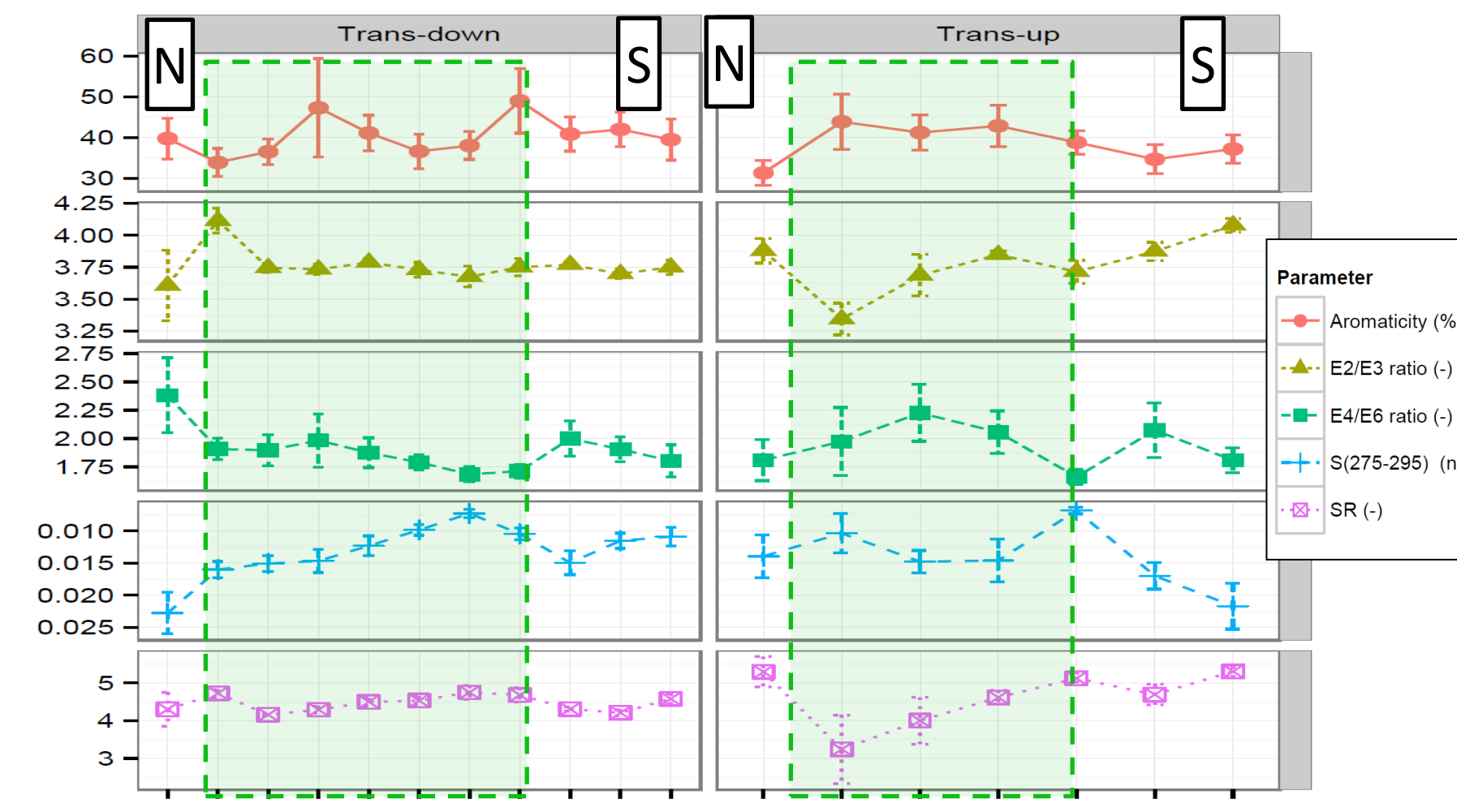
Fig. 10: Spatial variations in UV-VIS properties of DOM
