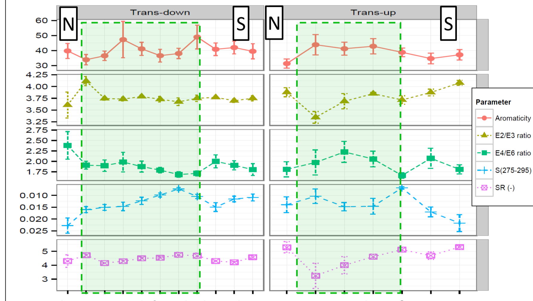
Fig. 10: Spatial variations in UV-VIS properties of DOM
