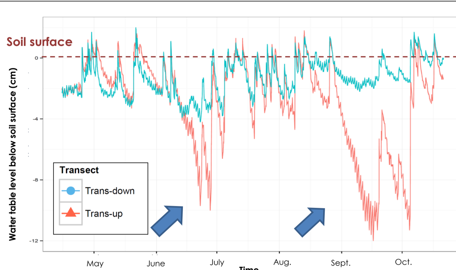
Fig. 2: Fluctuations of water table since restoration
