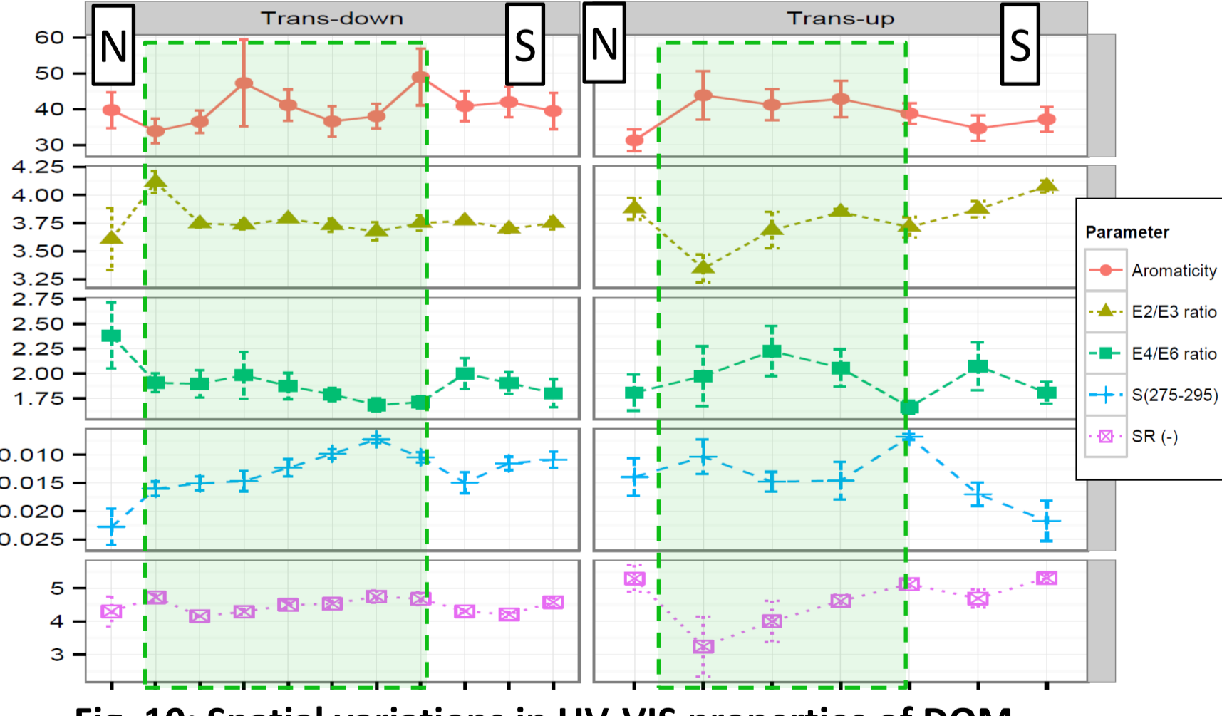
Fig. 10: Spatial variations in UV-VIS properties of DOM
