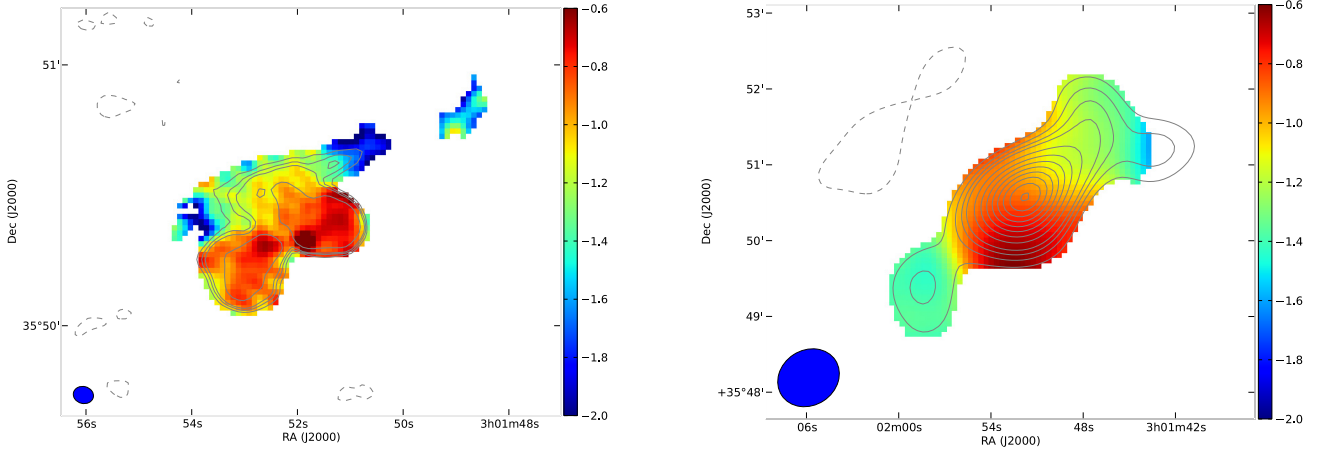
Fig. 5. Left: \alpha_{1415}^{4885} spectral index map of the inner lobes of 4C 35.06 using the archival VLA images listed in Table 1. Overlaid are VLA 4885 MHz contours ( -5, 18, 27, 36, 81\sigma ). Right: \alpha_{61}^{1360} spectral index map of the extended emission of 4C 35.06 using the LOFAR and WSRT images from this work. Overlaid are 33 contour levels from the LOFAR map spanning the range (-3, 183)\sigma . The beam sizes are given in the lower left corners.
