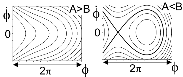
Figure 5. Phase portrait of the system (3).
