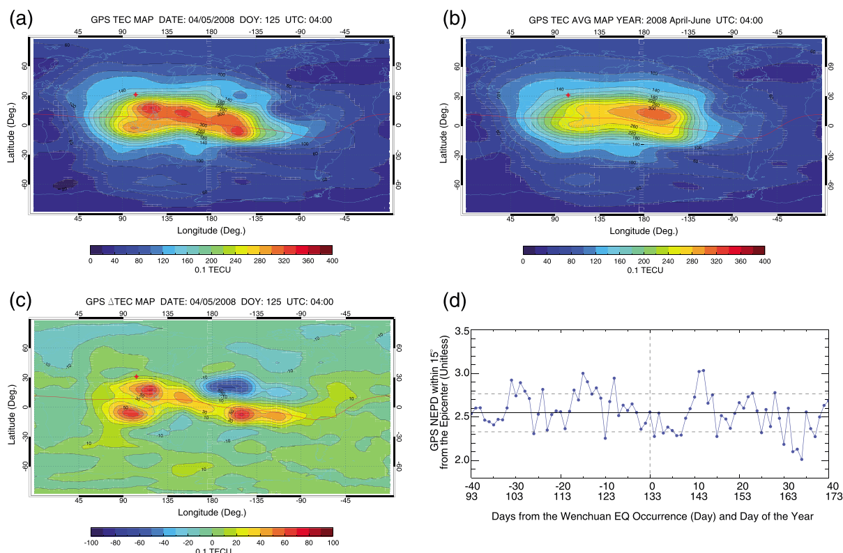
Figure 8. (a) GPS TEC map on 4 May 2008 (D-8) at 04:00 UTC, (b) averaged GPS TEC map of 04:00 UTC from April to June 2008, (c) \Delta TEC map ((a)-(b)) that illustrates the deviation of the TEC from the seasonal average on May 4, and (d) the daily evolution of the NEPD derived using the GPS TEC in the longitude range \pm 15^\circ from the epicenter at 04:00 UTC.
