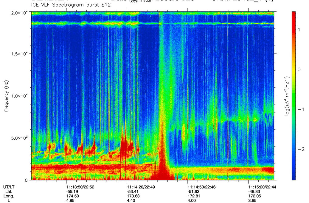
Figure 3. (top) Electric VLF spectrogram recorded on 14 January 2008 between 10:54:30 UT and 10:56:30 UT. (bottom) Electric VLF spectrogram recorded on 26 April 2008 between 11:13:35 UT and 11:15:35 UT. The spectrograms are from 0 up to 20 kHz, and their intensities are color coded according to the scales on the right. The parameters displayed below are the time in UT, the local time, the geographic latitude and longitude, and the McIlwain parameter L .
