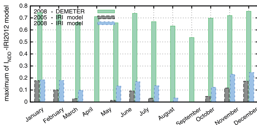
Figure 2. Comparison of maxima of I_{NDD} derived from IRI2012 for years 2005 (gray boxes) and 2008 (blue boxes) and in situ DEMETER data.
