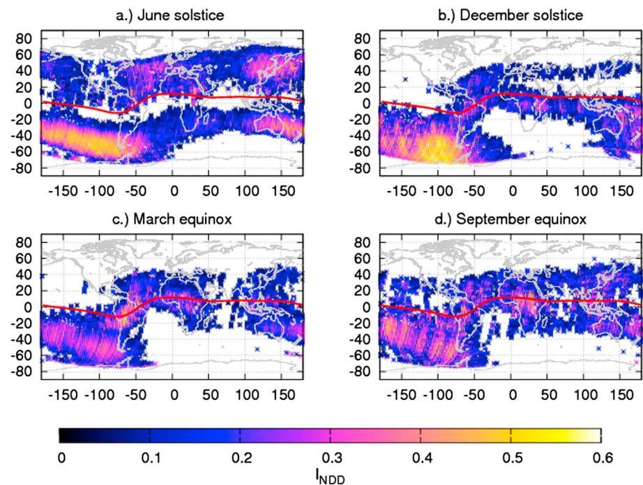
Figure 3. Averaged I_{NDD} > 0 plotted for (a, b) solstice and (c, d) equinox conditions.
