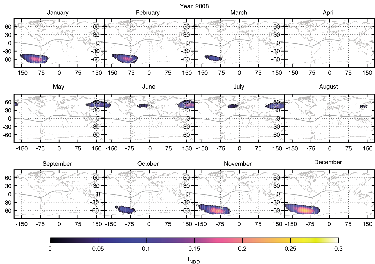
Figure 1. Monthly evolution of I_{NDD} index derived from synthetic data generated with IRI2012 model, year 2008. For the ease of identification of anomalous regions, only I_{NDD} > 0 is plotted.
