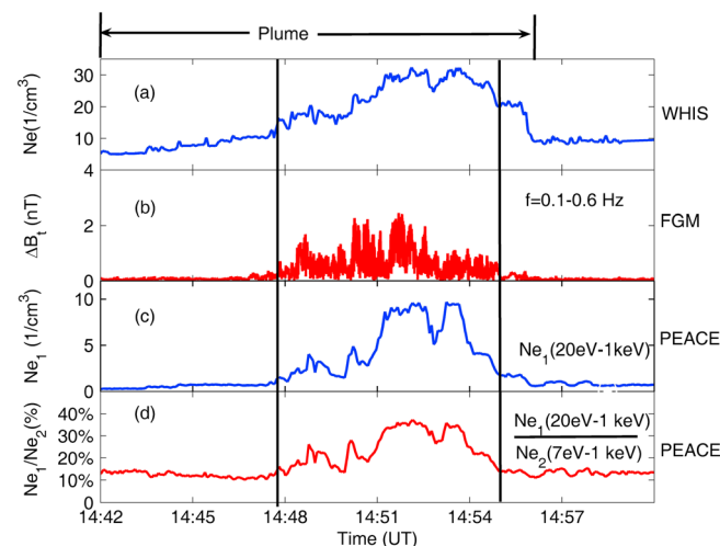
Figure 3. (a) Electron density measured by the WHISPER instrument. (b) Amplitude of perpendicular components ( \Delta B_t = \sqrt{\Delta B_{t1}^2 + \Delta B_{t2}^2} ) of disturbed magnetic field measured by FGM through a band-pass filter with a passband of 0.1–0.6 Hz in the field-aligned coordinates. (c) Electron density in energy range of 20 eV–1 keV detected by PEACE. (d) Ratio of electron density in energy range of 20 eV–1 keV to that in energy range of 7 eV–1 keV detected by PEACE. Two black vertical solid lines denote enhancements of the electron density in energy range of 20 eV–1 keV.
