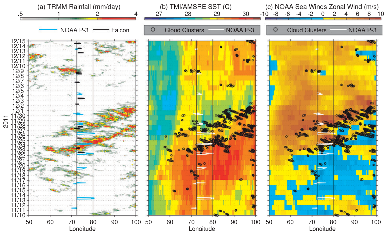
FIG. 2. Time–longitude diagrams of (a) TRMM 3B42 rain rate (color, mm day −1 ), (b) TRMM/AMSRE SST (color, °C) overlaid with cloud clusters from Meteosat-7 IR data, and (c) NOAA SeaWinds zonal surface wind (color, m s −1 ) from 10 Nov to 15 Dec 2011. The rain rate, SST, and zonal winds are averaged within the tropical latitude zone between 5°S and 5°N. The IR cloud clusters [cloud-top temperature < 208 K] are within the same latitude zone. The size of the black circles is proportional to the size of the observed cloud clusters. The DYNAMO-observing array is within the region between the blue lines (72°–80°E). The WP-3D aircraft tracks are marked in blue in (a) and white in (b) and (c). The Falcon 20 flight tracks are shown by black lines in (a).
