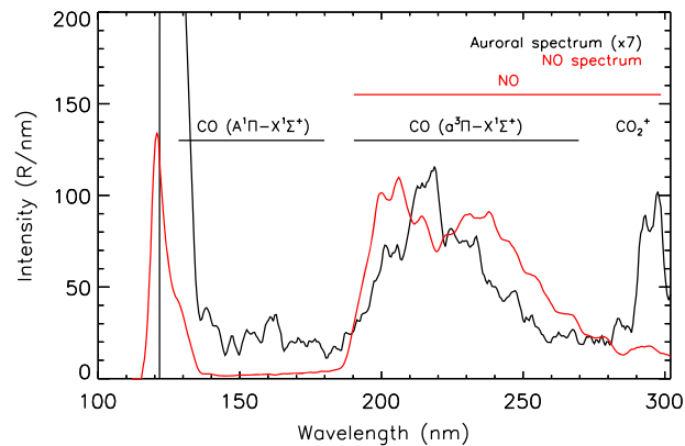
Figure 2. Spectrum measured at the nadir with the wide part of the SPICAM slit during the auroral detection of 19 February 2006 (black line). The spectral resolution is \sim 6 nm, and the data points have been smoothed over 5 pixels. The spectral regions of the CO Fourth Positive bands, the CO Cameron bands, and the \text{CO}_2^+ doublet are indicated. The broad feature on the left is the HI Lyman- \alpha line. For comparison, an average limb spectrum of the nitric oxide nightglow measured in the absence of auroral contribution during orbit 716 is shown by the red line (not to scale).
