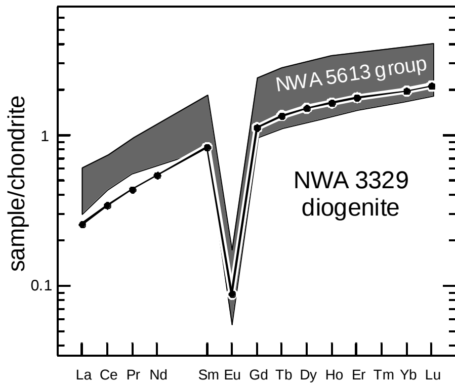
Fig. 8 CI normalized Rare Earth Element plot for the NWA 3329 diogenitic clast compared to some diogenites (NWA 5613 group, Barrat et al. 2010b).
