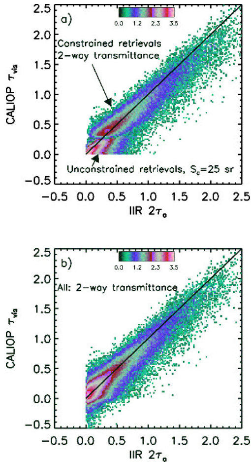
Fig. 1. 2D-histogram of nighttime CALIOP visible optical depth ( \tau_{\text{vis}} ) and 2\times IIR absorption optical depth at 12.05\ \mu\text{m} ( 2\tau_a ) with R_{\text{BG}} constrained by neighboring observations for single-layered semi-transparent cirrus composed of ROI (high confidence) over oceans during 2008. a) CALIOP version 3 products; b) for unconstrained retrievals, \tau_{\text{vis}} is from the apparent 2-way transmittance and not from S_c = 25\ \text{sr} . The black line represents \tau_{\text{vis}}/\tau_a = 2 . The color code is the decimal logarithm of the number of samples.
