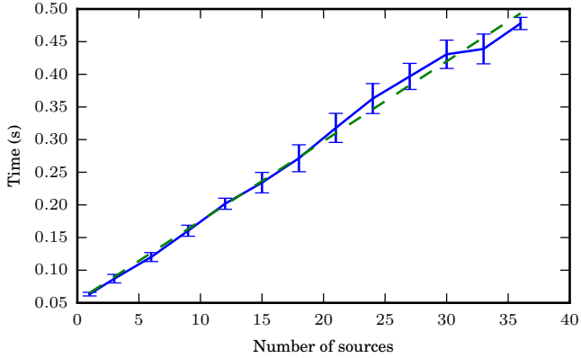
Figure 9: Time taken to find and measure the sources in an image as a function of the number of sources found. The solid line shows the mean time measured over 3800 test images; the dashed line a linear fit to the data.
