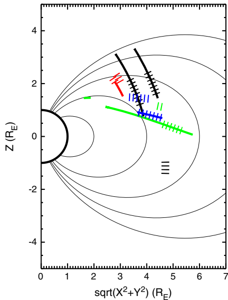
Figure 8. (a) Scheme of event locations in SM coordinates for which ULF magnetic field pulsations were observed simultaneously with the QP emissions. Altogether, ULF magnetic field pulsations were detected for four different QP events (11 June 2003 03:47–04:47 [black], 17 December 2006 01:12–01:17 [red], 13 April 2010 07:52–09:07 [green], and 22 April 2010 09:32–09:48 [blue]), the results obtained for each of them being plotted by a different color. The locations where QP electromagnetic emissions were observed are shown by thick solid curves. The locations where ULF magnetic field pulsations were observed are shown by periodic short transverse lines.
