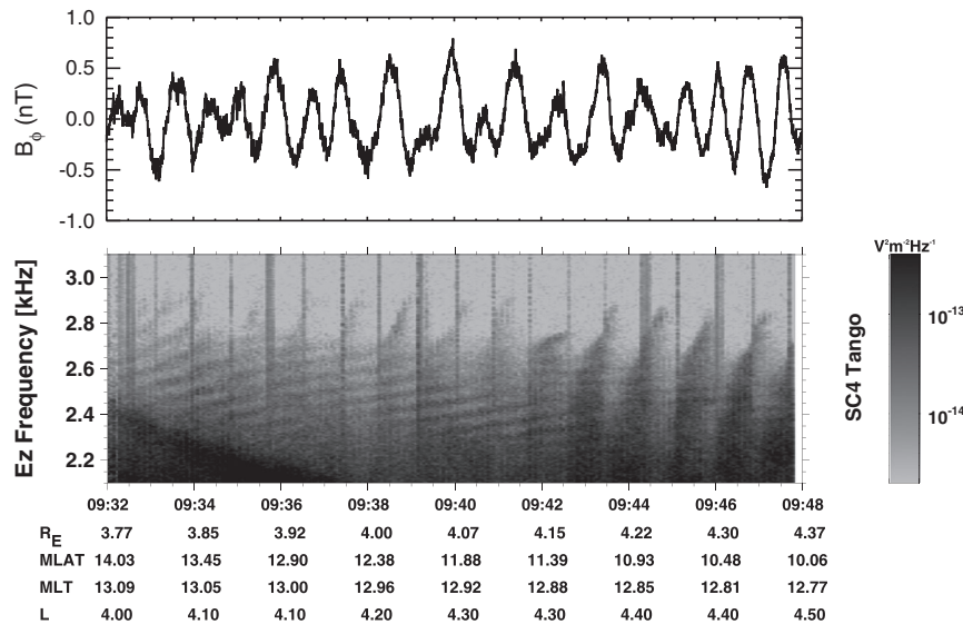
Figure 7. (top) ULF magnetic field pulsations measured by the FGM instrument on board Cluster 4 on 22 April 2010 between 0932:00 UT and 0948:00 UT. The plotted amplitude corresponds to the azimuthal direction, with a biquadratic fit subtracted. (bottom) Frequency-time spectrogram of power spectral density of electric field fluctuations measured by the WBD instrument on board Cluster 4 during the same time. The period of magnetic field pulsations is of the same order, but somewhat lower, than the modulation period of QP emissions.
