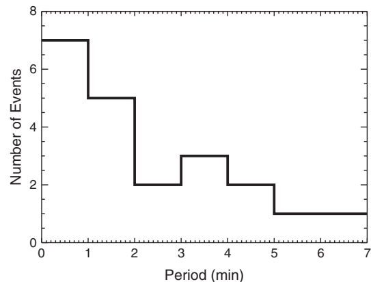
Figure 4. Histogram of overall modulation periods of QP events (see text).
