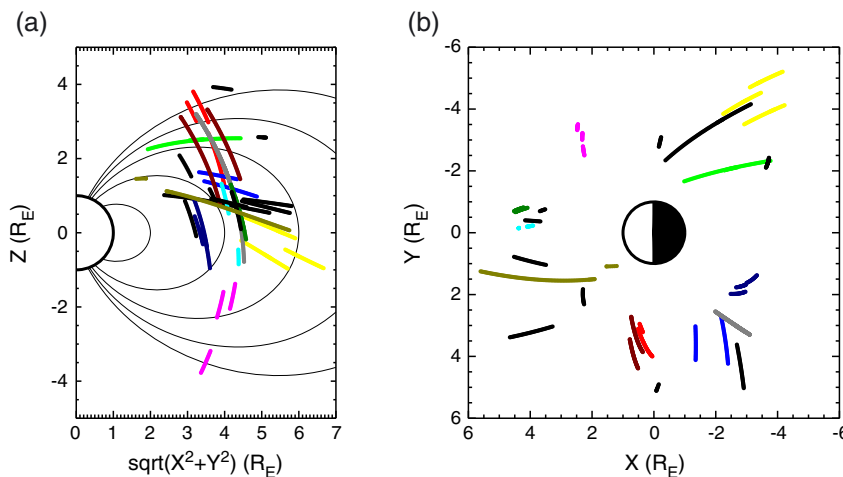
Figure 2. Locations of individual QP events in SM coordinates. (a) Meridional view. (b) Equatorial plane view. If an event was observed by a single Cluster spacecraft, it is plotted using the black color. If an event was observed simultaneously by several Cluster spacecraft, all the observations are plotted by the same (nonblack) color. Thin black curves in Figure 2a correspond to magnetic field lines with L = 2 , L = 4 , L = 6 , L = 8 , and L = 10 , inner to outer, respectively, calculated using the magnetic dipole model.
