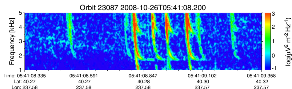
Figure 9. Frequency-time spectrograms of the power spectral density of electric field fluctuations measured in the Burst mode for typical whistler wave signatures. (a) Broadband signal of the fractional hop whistlers from about 1 to 5 kHz with no Earth-ionosphere waveguide cutoff present measured on 24 November 2007. (b) Fractional hop whistler with a cutoff at about 1.7 kHz observed on March 23, 2007. (c) The cutoff frequencies of the fractional hop whistlers at about 1.7 and 3.4 kHz observed on 26 October 2008.
