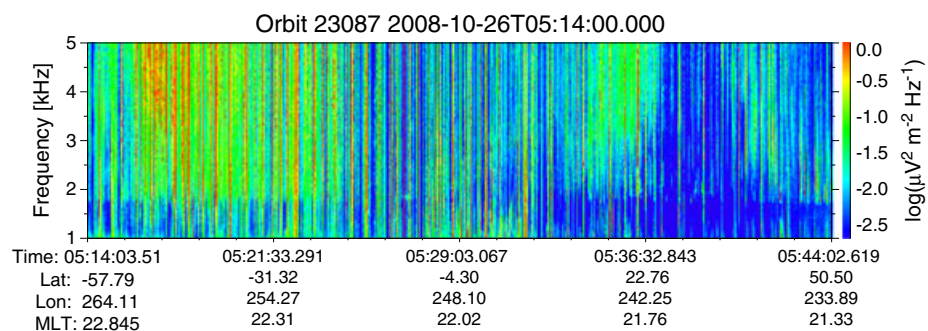
Figure 8. Frequency-time spectrogram of the power spectral density of electric field fluctuations observed by DEMETER on 26 October 2008 between 05:14 and 05:44 UT . Note the whistler cutoff frequency of the whistlers (vertical lines) at about 1.7 kHz. The cutoff frequency remains nearly constant at all of the sampled latitudes.
