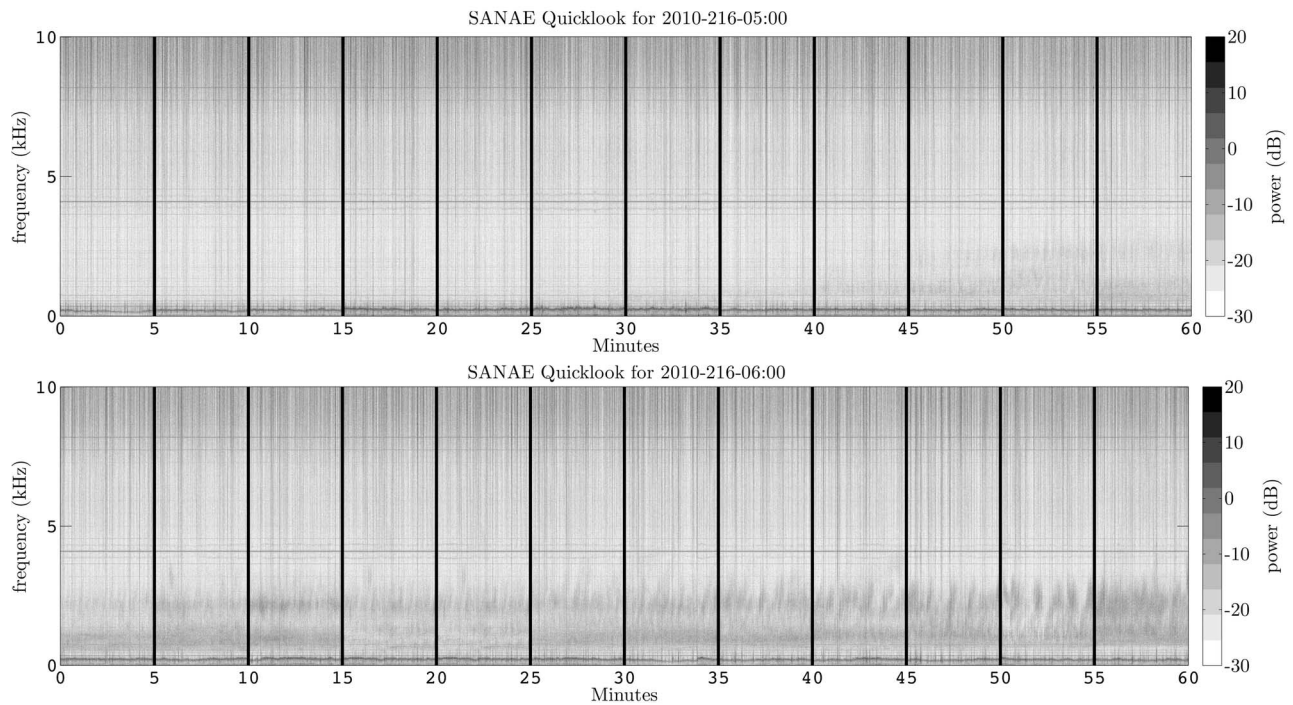
Figure 6. VLF spectrograms at SANA E IV from 05:00–07:00 UT on 4 August 2010. The format is the same as Figure 1. There is chorus for the duration of these spectrograms. This chorus spans a different frequency range, and occurs at a later UT than the Marion Island chorus.
