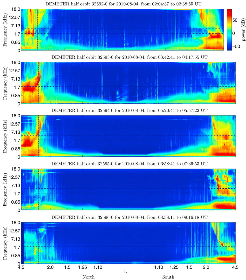
Figure 13. Broadband VLF data from the 5 descending DEMETER half orbits shown in Figure 11. The vertical dotted lines are the L -value of Marion Island ( L = 2.60 ) in both hemispheres, and the horizontal dotted lines represent the frequency envelope of the chorus observed on Marion Island.
