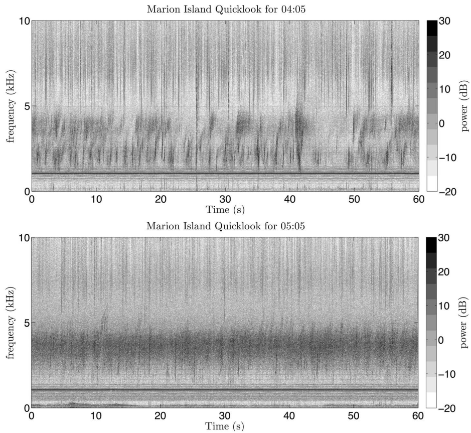
Figure 2. Detailed spectrograms of the (top) chorus (at 04:05 UT) and (bottom) hiss (at 05:05 UT). The structure of the chorus elements is visible in the top panel, and in the bottom panel, one can see that chorus elements are still present beneath the hiss.
