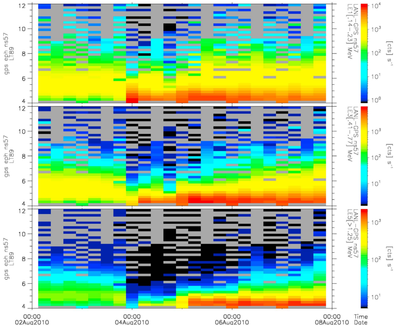
Figure 5. Electron flux data obtained from detectors on LANL GPS satellite NS57 in the range from L = 4 – 12 , in three energy channels. There is a depletion in the radiation levels at the time of the storm onset, and an increase in density at 4 \leq L \leq 5 for the next few days.
