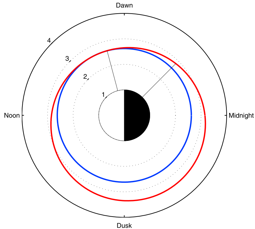
Figure 9. Polar plot of the equatorial plasmopause location obtained from the empirical model in equation (2) (red), and the L -shell of Marion Island mapped into the equatorial plane (blue). The radial black lines show MLT of the period for which chorus was observed at Marion Island. This indicates that the plasmopause was very likely close to Marion Island during the event.
