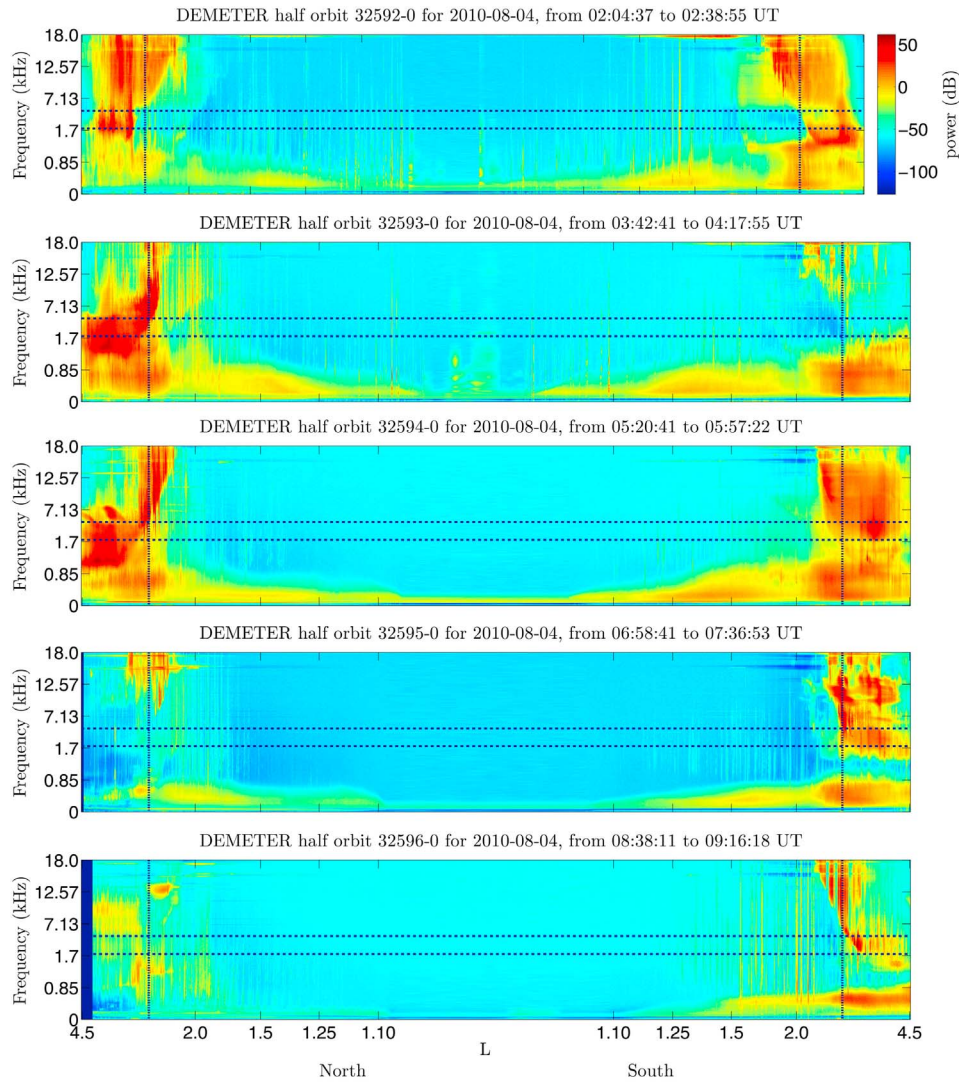
Figure 16. Residuals after a subtraction of the mean of the DEMETER data presented in Figure 13. The chorus is much more evident in these plots. The vertical lines show the L -value of Marion Island in both hemispheres. The two horizontal lines show the frequency range 2–5 kHz.
