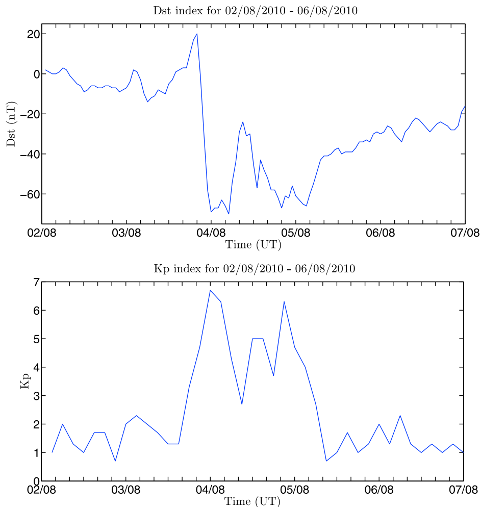
Figure 4. The Dst and K_p indices from 2 to 7 August 2010. The signature of a geomagnetic storm is evident in Dst at 00:00 UT on 4 August 2010, 3 hours before the onset of the chorus at Marion Island. There is a rapid increase in K_p at this time.
