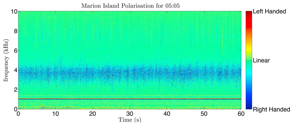
Figure 12. Polarization of the signal received at Marion Island for the minute 05:05 UT. Note the strong right handed polarization of both the chorus and the hiss, indicating a nearby entry into the EIWG.
