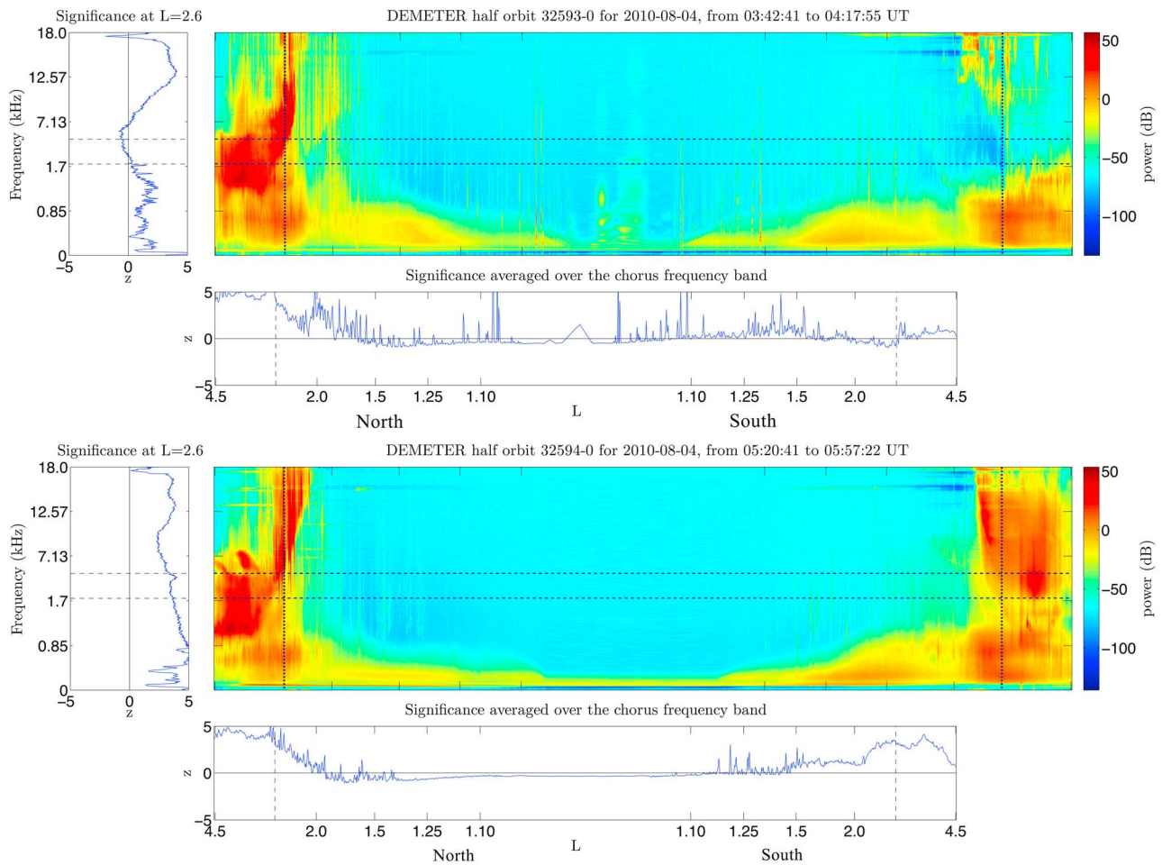
Figure 15. Residual for descending DEMETER half orbits 32593 and 32594. The left hand plots show the z -value obtained at the magnetic latitude of Marion Island. The bottom plots show the z -value averaged over 2–5 kHz. The z -value is large during periods of high chorus activity, and small during periods of no chorus.
