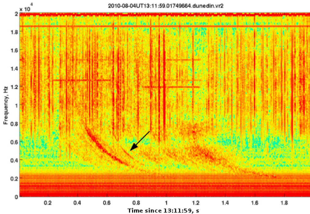
Figure 10. The knee whistler observed at Dunedin on 4 August 2010. The origin of the time axis is 13:11:59 UT. The knee whistler is the well defined trace at approximately 0.8 s, indicated by the arrow.
