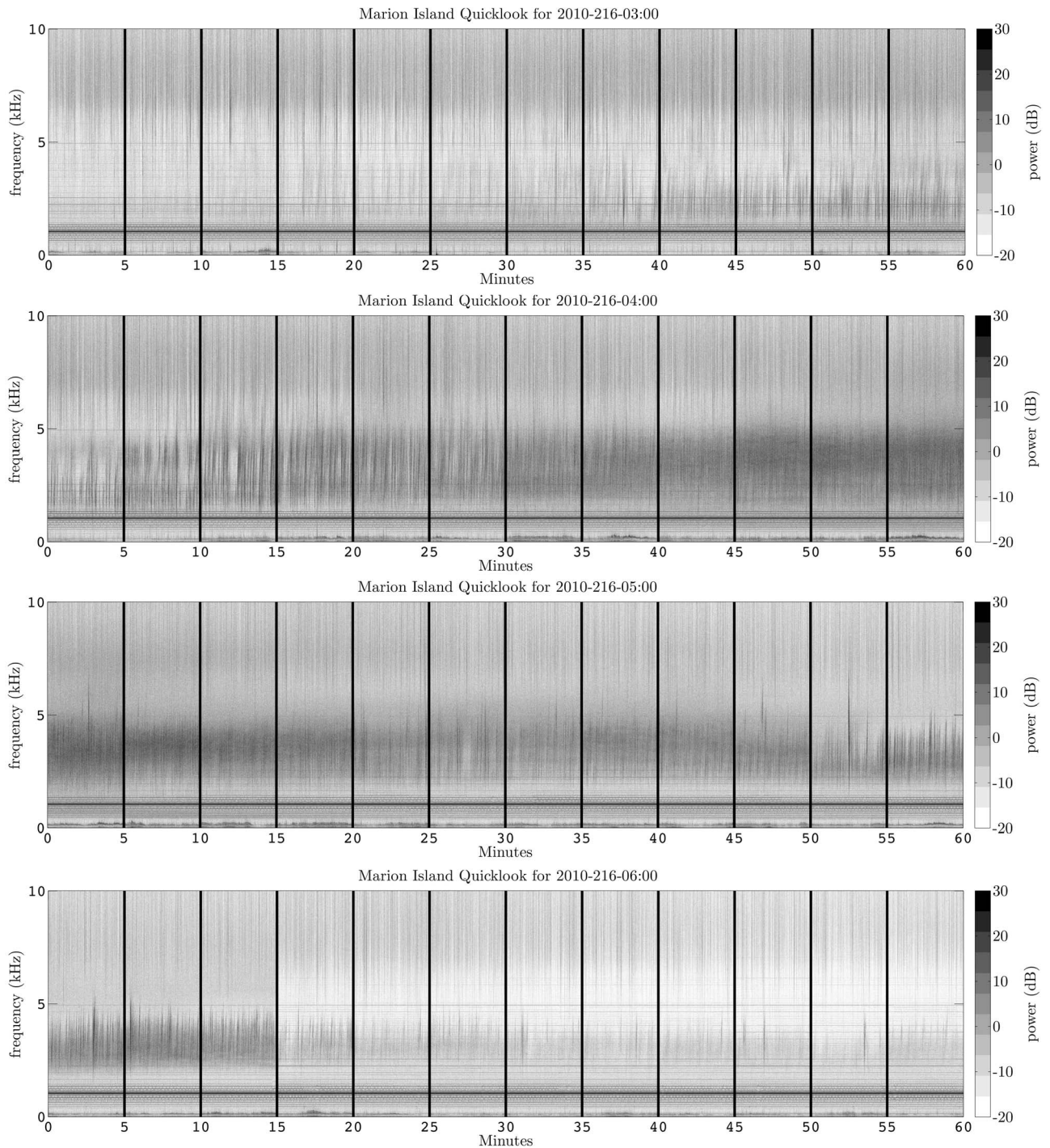
Figure 1. The evolution of chorus at Marion Island over 4 hours from 03:00–07:00 UT on 4 August 2010 with time resolution of 50 ms. Each plot represents 1 hour of data, and each vertical slice represents 1 minute of data sampled every 5 min. The chorus transforms into hiss at 04:30 UT, which evolves to chorus at 05:50. There are changes to the upper boundary of the frequency envelope during the evolution.
