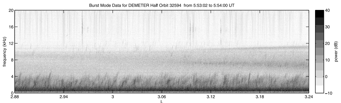
Figure 14. Burst mode VLF data from DEMETER satellite half orbit 32594 which shows chorus being observed. This data is for a one minute period while the satellite was in the southern hemisphere. The position of this spectrogram relative to those plotted in Figure 13 can be inferred from the L -values.
