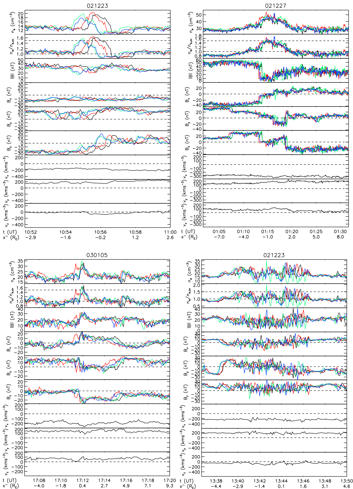
Figure 3. Cluster data from four encounters of density enhancements. From top to bottom the panels show electron density, ratio of electron density to background density, total magnetic field, the three components of the magnetic field in GSE coordinates, and the three components of the drift velocity in GSE coordinates. The color coding is the same as in Figure 1. For the velocity only the data from S/C 1 is shown.
