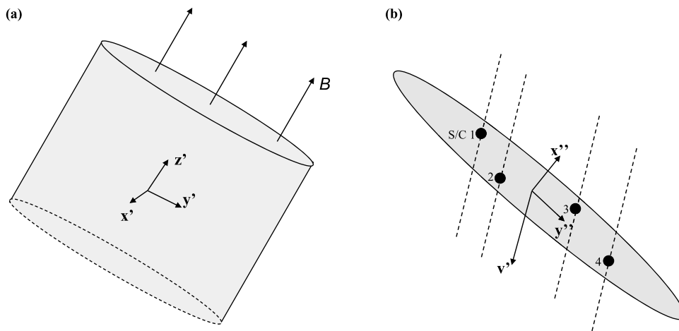
Figure 5. (a) Schematic representation of coordinate system used in minimum variance analysis. (b) Schematic of the probing of the plasmoid as it sweeps across the spacecraft.
