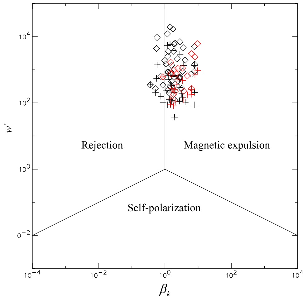
Figure 11. Plasmoid parameters in the parameter space defined by Brenning et al. [2005]. w' is a normalized width of the plasmoid (see text for definition), and \beta_k is the kinetic beta, evaluated with the directed velocity of the plasmoid, and with the magnetic field inside the magnetosphere. The mechanisms of the different regions pertain to the situation of penetration at the boundary of the high magnetic field region. See also text for explanation of symbols. The same color coding as in Figure 9 is used.
