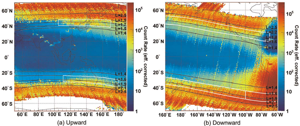
Figure 2. Electron flux distribution with the energy in the range of 108–411 keV during the whole year of 2008. Color scales indicate the average flux value within a pixel size of (1°, 1°). The simplified unit of counting rate (counts/s) is obtained by multiplying the factor of 1.16 (cm 2 sr) with the averaged flux value.
