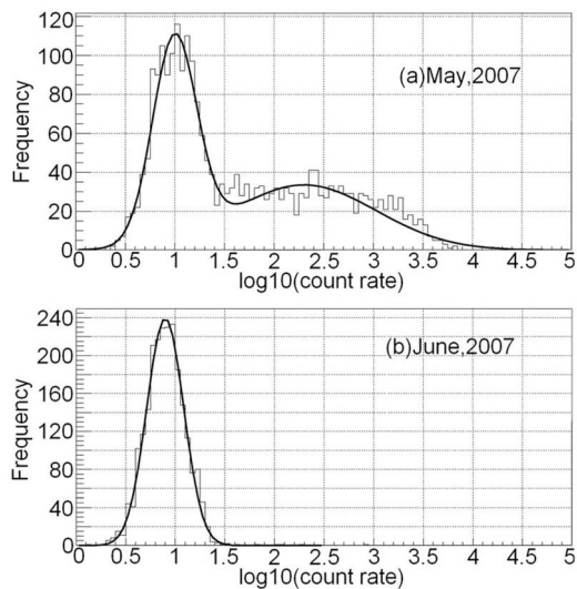
Figure 3. Statistical distribution of electron flux on logarithmic scale, for local data (NL and SL) with an energy band of 206 \pm 26.7 keV. The distribution in May has one more component with higher flux comparing with the one in June.
