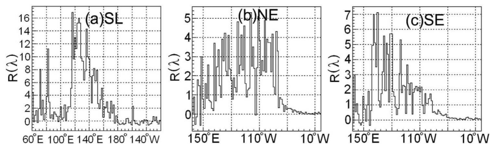
Figure 8. Ratio of signal to background R(\lambda) versus geolongitude in the regions (a) SL, (b) NE, and (c) SE.
