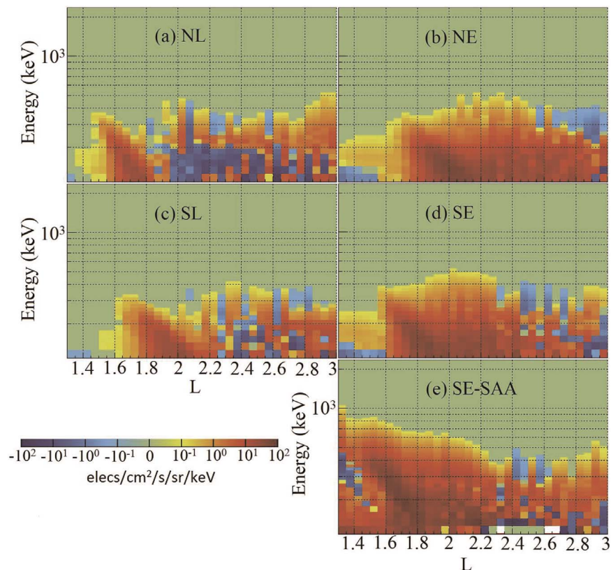
Figure 10. Spectrogram of the NWC electrons along with L values in five different regions. Figure 10e is for the SE-SAA region, which is an extension of the SE range with longitude of ( 100^{\circ}\text{W} – 60^{\circ}\text{W} ). Blue corresponds to a flux of (on-off) < 0 . Here we set zero for |flux| \leq 10^{-2} el \text{cm}^{-2} \text{s}^{-1} \text{sr}^{-1} \text{keV}^{-1} . Data with only statistical fluctuation have been ignored.
