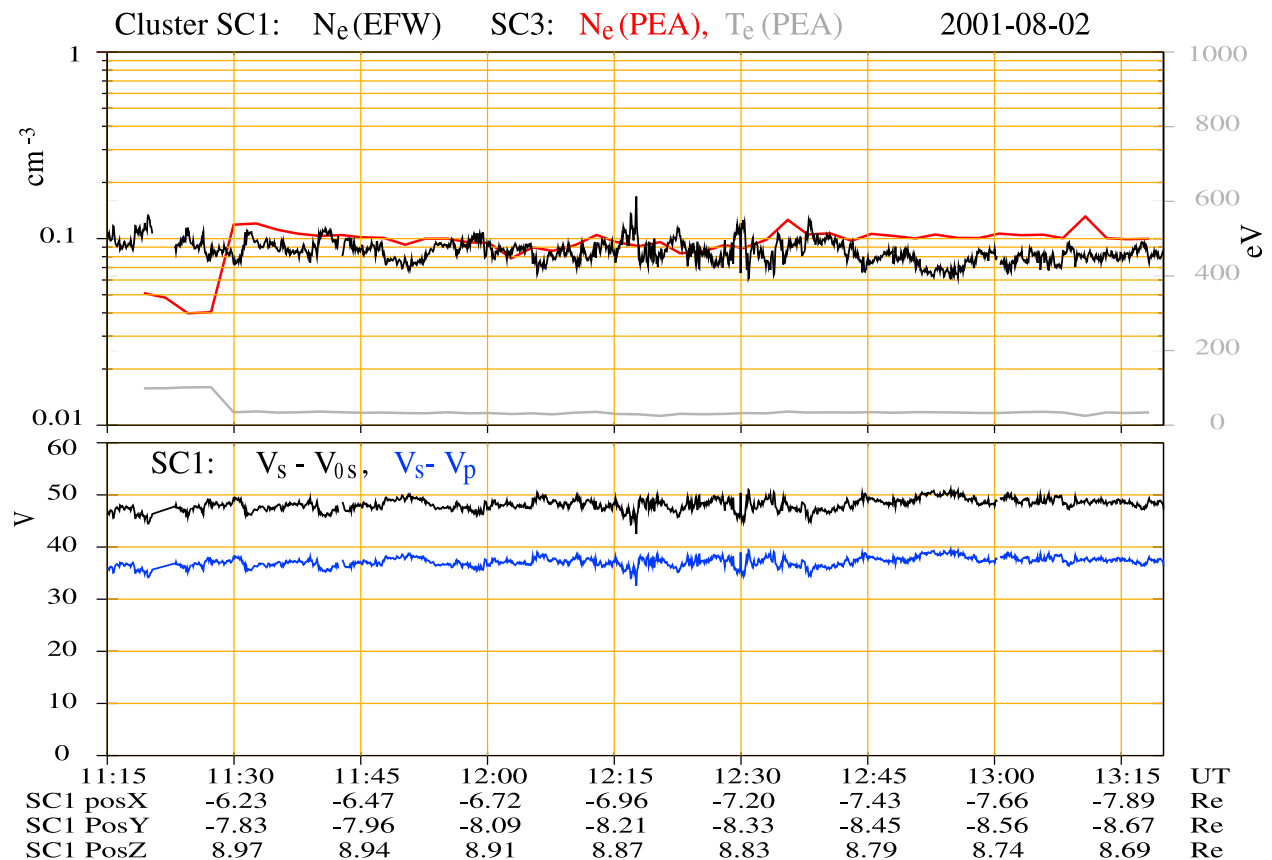
Figure 11. Another opportunity to test N_e(\text{EFW}) in a tenuous polar cap – lobe plasma appeared when ASPOC controlled C3 and C4 to be at a potential relative to the ambient plasma of less than 10 V. PEACE could then measure a more complete electron spectrum. C1 had no ASPOC operation. The Cluster satellites were at (13–14) R_E , and all had nearly identical values of (V_s - V_p) before and after ASPOC being active on C3. This indicates that all satellites were in the same plasma during the time period presented, and it is possible to demonstrate agreement between N_e(\text{EFW}) on C1 and N_e(\text{PEACE}) on C3.
