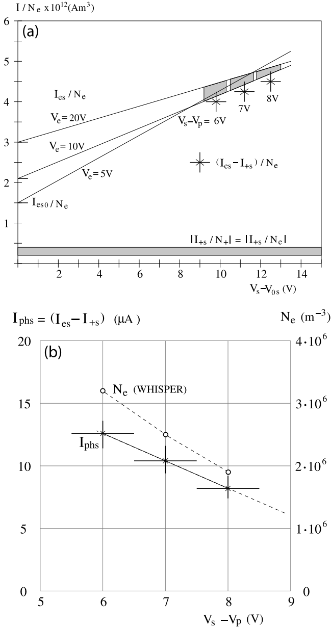
Figure 4. (a) I_{es}/N_e as a function of (V_s - V_{0s}) can be calculated for Cluster from equation (2) for different values of V_e . We assume that a safe range for V_e in the solar wind is from 5 V to 20 V. The linear functions of I_{es}/N_e tend to focus near values of (V_s - V_{0s}) corresponding to values of (V_s - V_p) in the range (6–8) V. By correcting for a small ion current, I_{+s} in the solar wind, we can find (I_{es} - I_{+s})/N_e , which in turn can be used to find the current of escaping photoelectrons, I_{phs} = (I_{es} - I_{+s}) when N_e data is available. (b) For January–March 2006 the (0–105) nm solar radiation was stable at 3 \text{ mWm}^{-2} for longer periods. N_e data from WHISPER, combined with (I_{es} - I_{+s})/N_e in Figure 4a, could then be used to find I_{phs} versus (V_s - V_p) and demonstrates that I_{phs} increases with approximately 20% per volt when (V_s - V_p) changes from 8 V to 6 V.
