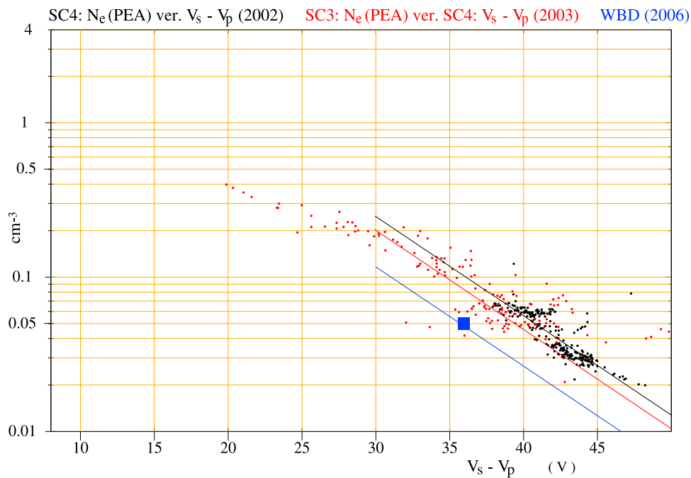
Figure 7. In the autumn of 2003 all Cluster spacecraft were separated by a few hundred km in the cusplolar cap, and often all spacecraft showed near identical values of (V_s - V_p) , indicating that all were in the same plasma. This opened for the possibility to get N_e based on PEACE full spectrum measurements during ASPOC operations on C3, and at the same time get (V_s - V_p) from C4 with no ASPOC operations. The red dots are the result of such measurements during selected periods. The black dots are from a particular event in the lobe in 2002. See Figure 10 and related text. The small square near (V_s - V_p) = 36 V is a WBD determination of N_e from a measurement of a cut-off frequency in 2006. The red, black and blue lines are starting at (V_s - V_p) = 30 V from N_e values in Figure 6.
