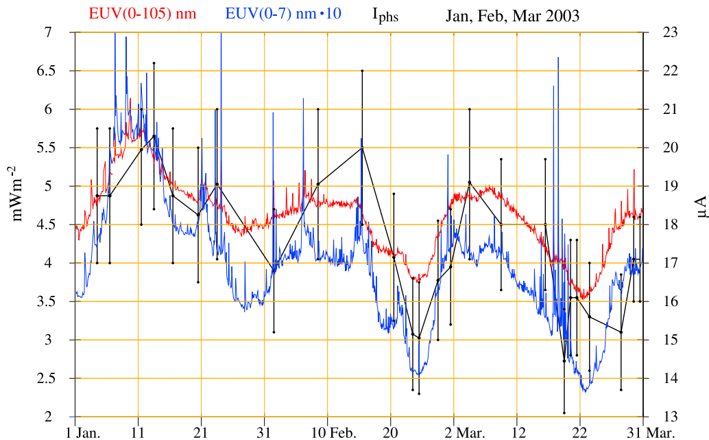
Figure 5. The red curve is the (0–105) nm, and the blue curve the (0–7) nm solar EUV radiation for January–March 2003. I_{\text{phs}} = I_{\text{es}} - I_{\text{+s}} for (V_s - V_p) = (7 \pm 5) V is presented for 25 solar wind events when I_{\text{phs}} could be determined based on WHISPER measurements. This demonstrates that I_{\text{phs}} is controlled by the solar EUV radiation.
