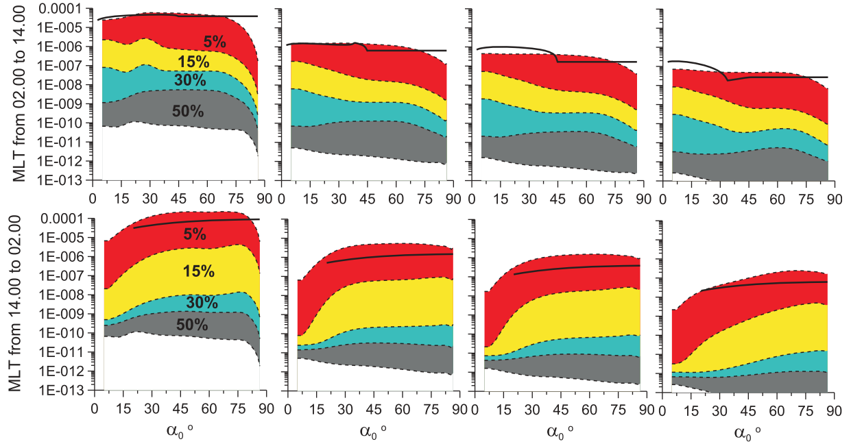
Figure 2. Distribution of energy diffusion coefficients \langle D_{EE}/E^2 \rangle \text{s}^{-1} for \Omega_{pe}/\Omega_{c0} = 4.5 and four energies ( E = 0.1, 1, 2, and 5 MeV from left to right). Red color corresponds to the range of \langle D_{EE}/E^2 \rangle variation for the most intense waves with 5% probability; \langle D_{EE}/E^2 \rangle can be found inside yellow, blue and grey ranges for less intense waves ranges corresponding to 15%, 30% and 50% probabilities, respectively. For the calculation of \langle D_{EE}/E^2 \rangle the effect of B_w variation with \lambda is also taken into account. The B_w distributions correspond to high geomagnetic activity K_p > 5 (see details of chorus distributions in Artemyev et al. [2012b]). The (top) dawn/day and (bottom) dusk/night sectors. Black solid curves show \langle D_{EE}/E^2 \rangle estimates (14), (16), and (17) for 60 pT chorus waves.
