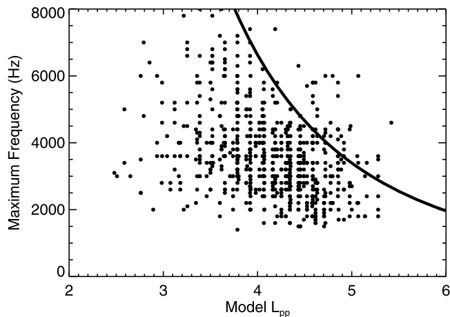
Figure 9. Maximum frequency of MLR events as a function of the model location of the plasmopause. One half of the equatorial electron cyclotron frequency at the plasmopause distance is over-plotted by the thick solid line.
