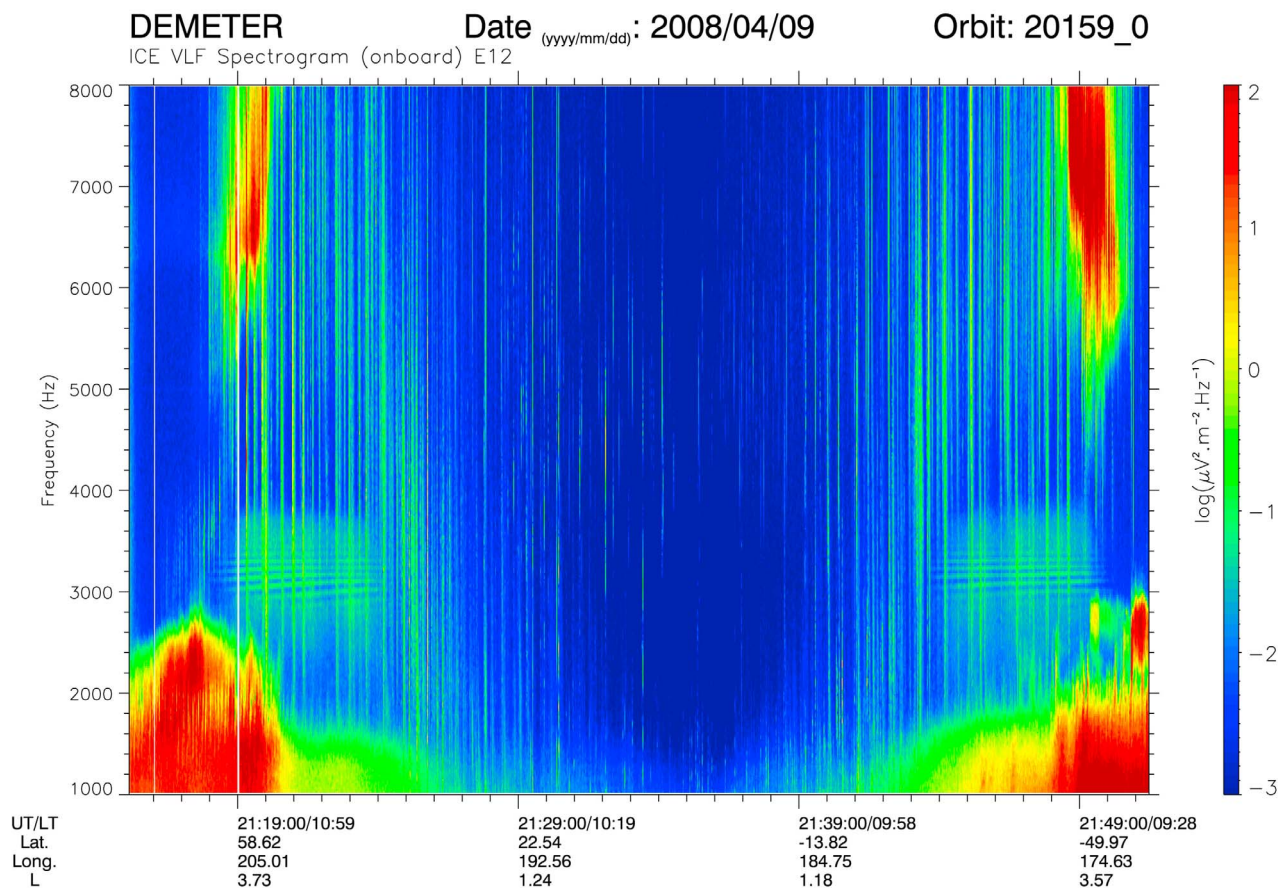
Figure 1. An example of a frequency-time spectrogram of a single half-orbit used for the identification of magnetospheric line radiation (MLR) events. Two MLR events at frequencies between about 2800 and 3400 Hz can be seen. The first MLR event was detected between about 21:19 UT and 21:24 UT. The second MLR event was detected between about 21:44 UT and 21:49 UT. The events occur close to the magnetically conjugate regions.
