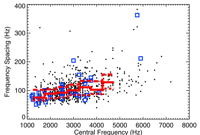
Figure 5. Frequency spacing of individual lines forming the events as a function of their central frequency. The format of the figure is the same as that of Figure 3b.
