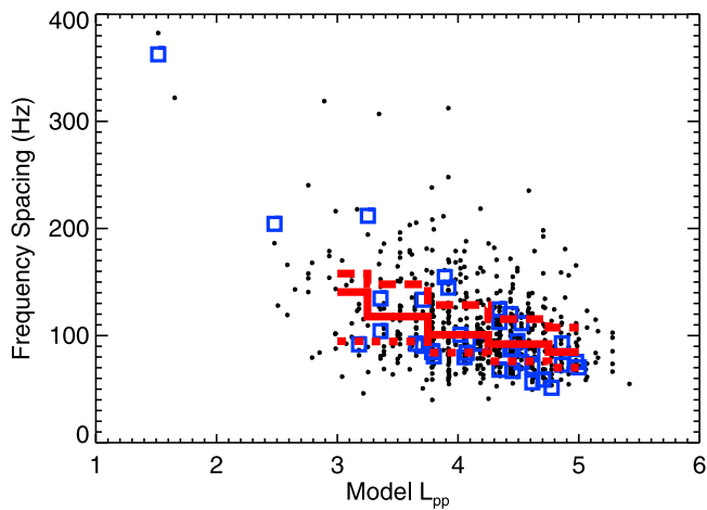
Figure 8. Frequency spacing of the individual lines forming the events as a function of the model location of the plasmapause. The format of the figure is the same as that of Figure 3b.
