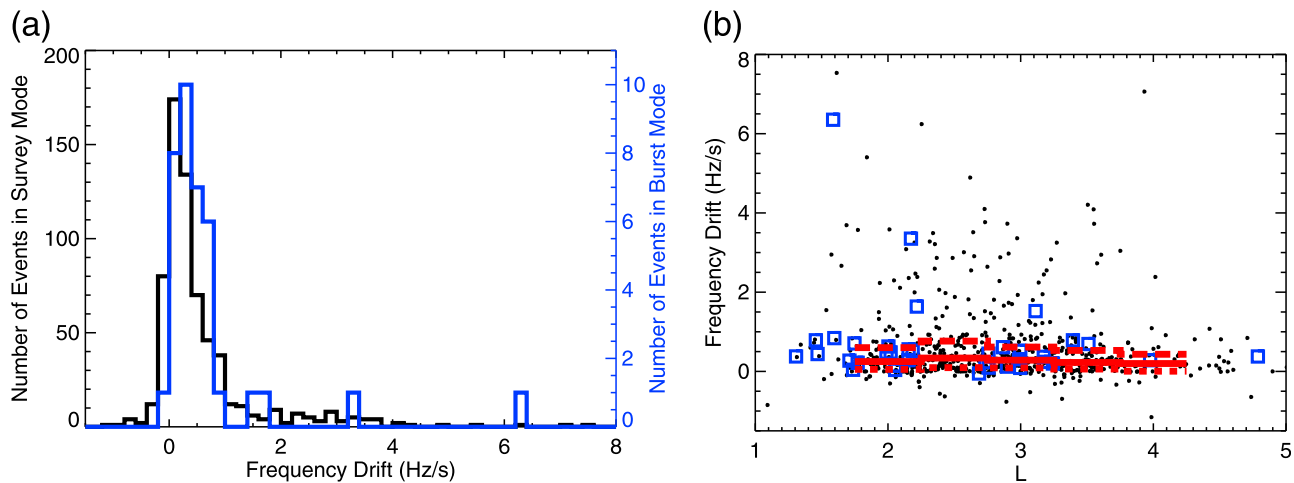
Figure 4. (a) Histograms of average frequency drifts of the analyzed events. The histogram obtained using the survey mode data is plotted by the black line, using the scale on the left. The histogram based on a few events for which the burst mode data were available is plotted by the blue line, using the scale on the right. (b) Average frequency drift of the events as a function of their central L-shell. The format of the figure is the same as that of Figure 3b.
