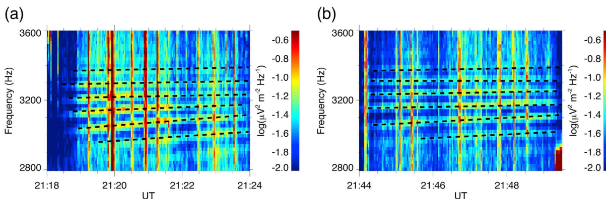
Figure 2. Detailed frequency-time spectrograms corresponding to the two MLR events from Figure 1. The straight lines manually found to approximate the individual lines forming the events are over-plotted by the black dashed lines.
