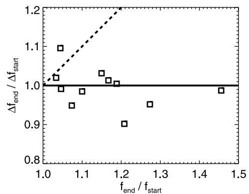
Figure 7. Ratio of the frequency spacing at the end and at the beginning of 11 MLR events that are formed by the lines whose frequencies increase significantly over the time duration of the events as a function of the relative change of their frequency. The dashed line shows the dependence expected for the generation at harmonics of the base frequency equal to the frequency spacing. The solid line shows the dependence corresponding to a constant frequency spacing.
