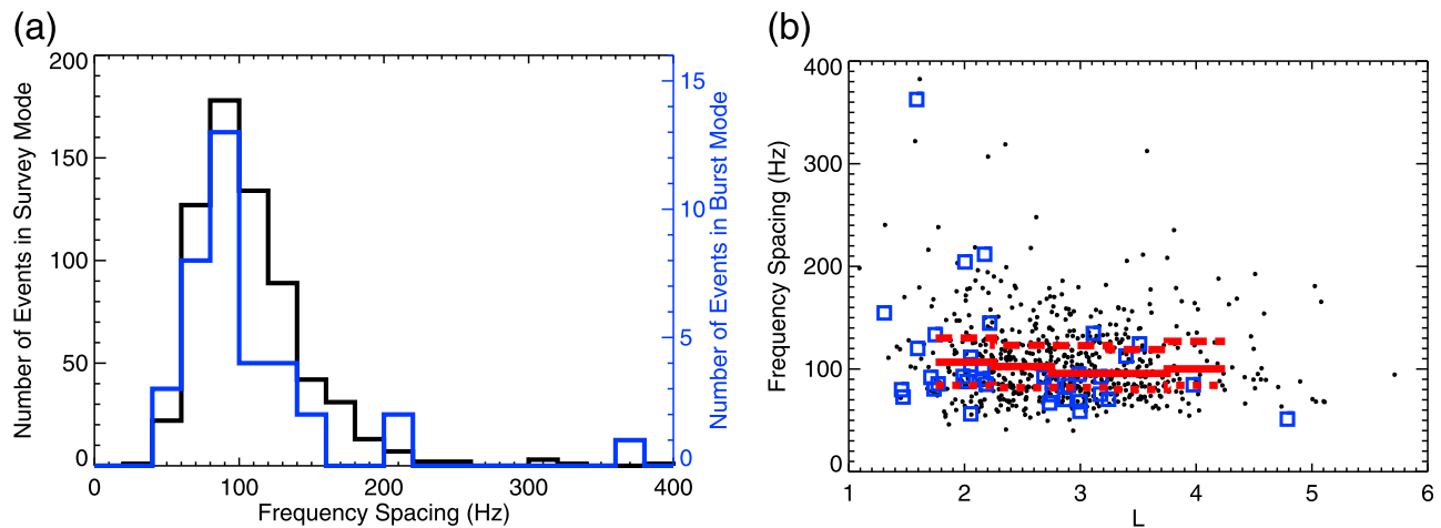
Figure 3. (a) Histograms of frequency spacing of individual lines forming the events. The histogram obtained using the survey mode data is plotted by the black line, using the scale on the left. The histogram based on 37 events for which the burst mode data were available is plotted by the blue line, using the scale on the right. (b) Frequency spacing of individual lines forming the events as a function of their central L-shell. The results obtained using the survey mode data are plotted by the black points. The results obtained for a few events for which the burst mode data were available are plotted by the blue squares. The red lines show the median value (solid) and the 0.25 and 0.75 quartiles (dotted and dashed, respectively).
