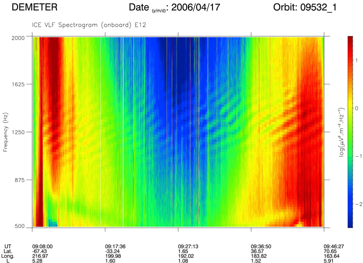
Figure 6. Frequency-time spectrogram of an MLR event that is formed by the lines whose frequencies increase significantly over the time duration of the event.
