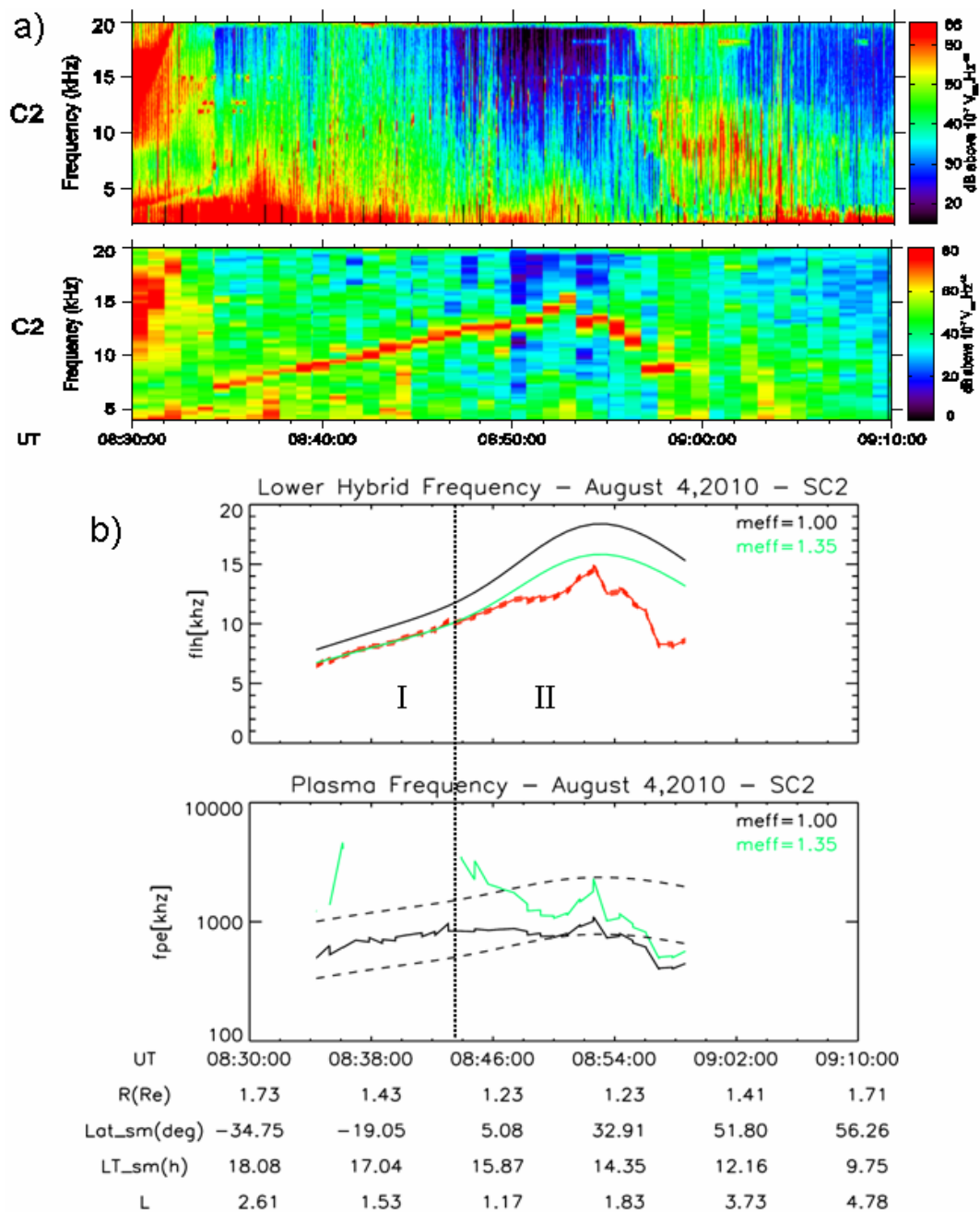
Fig. 6. Analysis of F_{\text{lh}} measurements on the C2 satellite, for the 4 August 2010 case event. (a) Frequency time spectrograms from the WHISPER instrument. Top: active and passive spectra. Bottom: active spectra. (b) Same parameters and presentation as panels (b) and (c) in Fig. 5.
