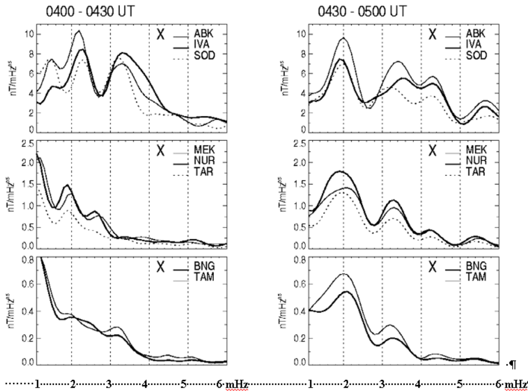
Fig. 1. Spectra of the geomagnetic pulsations at polar and lower latitude stations along geomagnetic meridians of about 107^{\circ} – 110^{\circ} , concerning sequence 1 (left: 04:00–04:30 UT) and sequence 2 (right: 04:30–05:00 UT) (part of Fig. 4 in Manninen et al., 2010).
