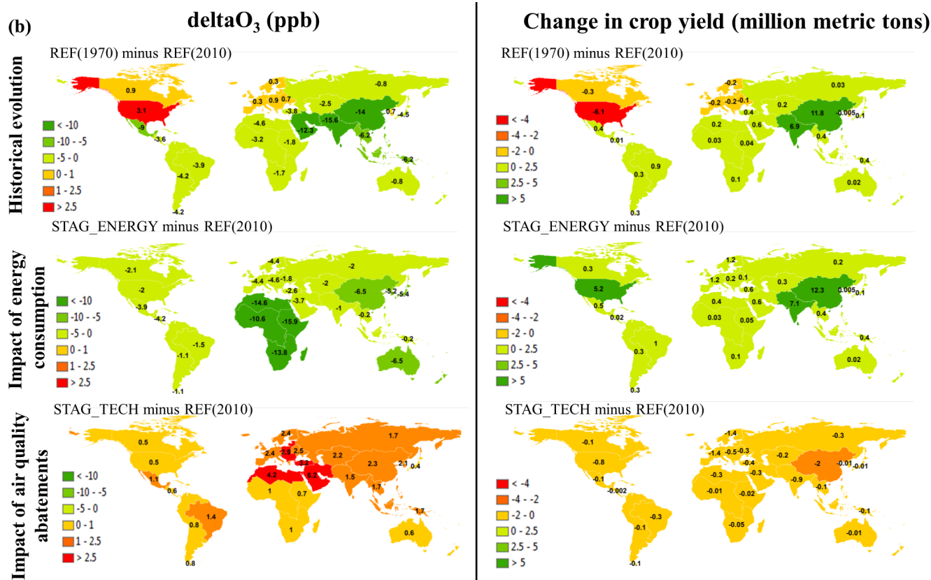
Figure 10. Relative change between the scenarios (STAG_ENERGY, STAG_TECH and REF(1970)) and the reference case (REF(2010)): regional change in (a) \text{PM}_{2.5} ( \mu\text{g m}^{-3} ) and associated life expectancy (months) and (b) in ozone mixing ratios (ppb) and associated impacts on crops. Note that the same color scales are used for \text{deltaPM}_{2.5} and \text{deltaO}_3 (positive delta are associated with red colors representing bad impacts, while negative delta are in green colors representing improvements). Opposite color scales are applied for change in life expectancy and crop yield compared to the delta one (positive values are reported in green and negative values in red representing good and bad impacts, respectively).
