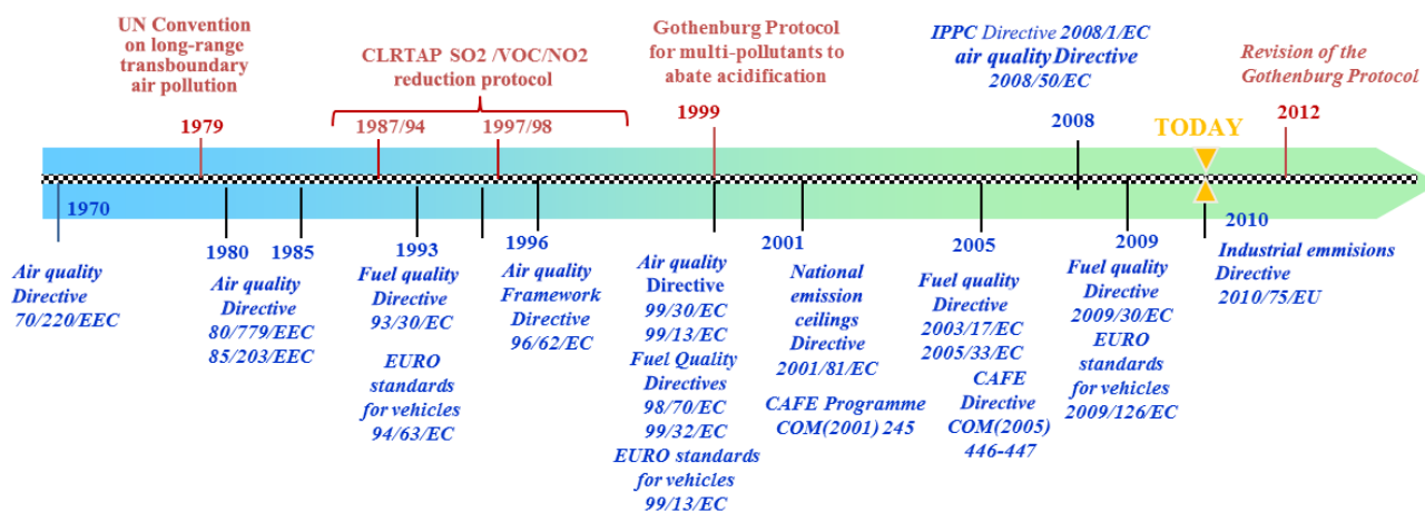
Figure 1. Overview of historical European Union (in blue) and international (in red) air quality regulations. UNECE/CLTRAP covers all European countries, USA, Canada, Belarus, Russia, Turkey, Israel, Ukraine, and central Asian states.
