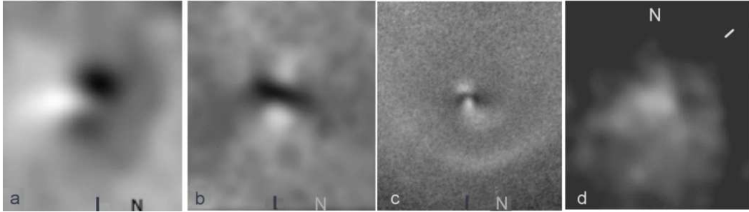
Figure 8: Evidence for different properties of solid particles in different regions of cometary comae, from linear polarization (P) maps at a given phase angle ( \alpha ) a. Comet C/1990 K1 Levy at \alpha = 18^\circ , in a field of view of 4000 km by 4000 km (black, P = -2.6\% ; white, P = 0.5\% ). b. Comet C/1995 O1 Hale-Bopp at \alpha = 7^\circ , in a field of 38000 km by 38000 km (black, P = -6\% ; white, P = 2\% ). c. Comet Hale-Bopp, now at \alpha = 44^\circ , in a field of 82000 km by 82000 km (black, P = 9\% ; white, P = 18\% ). d. Comet 9P/Tempel 1, before Deep Impact event, without any conspicuous feature, at \alpha = 41^\circ , in a field of 70000 km x 70000 km (black, P = 1\% ; white, P = 10\% ). The solar direction is indicated by a black or white tick.
