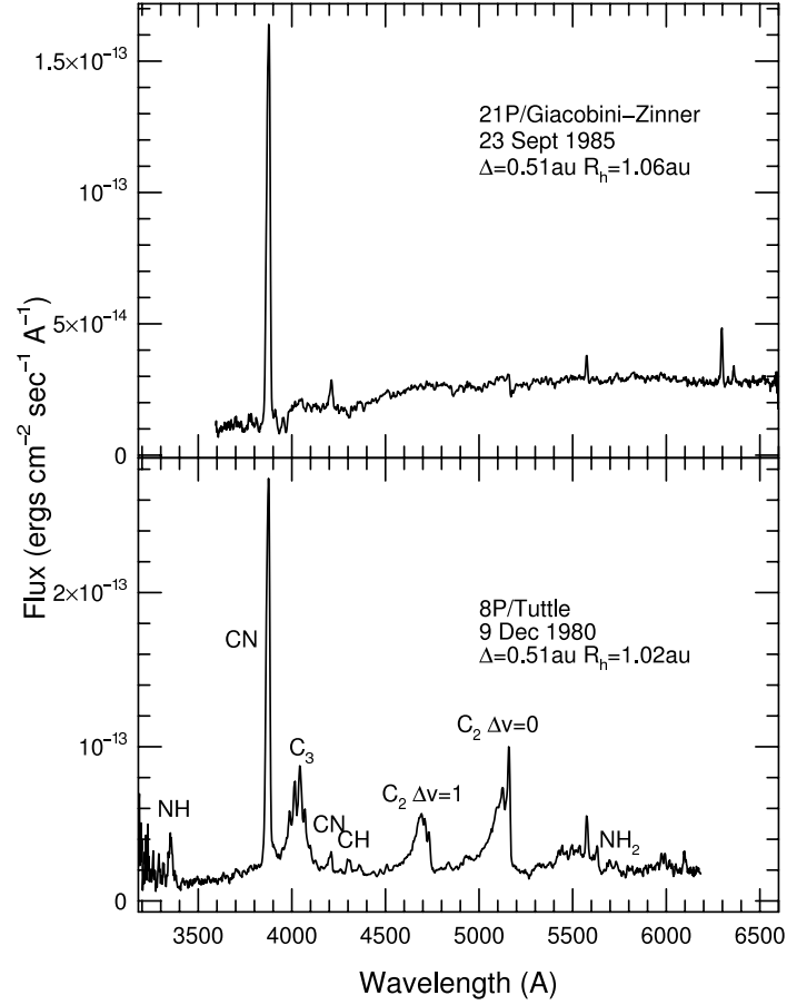
Figure 1: Spectra of 21P/Giacobini-Zinner and 8P/Tuttle obtained at McDonald Observatory are shown, scaled to the CN band at 3880Å. The comets were observed at comparable heliocentric and geocentric distances. Inspection of the figure shows that the well-defined C 2 and C 3 bands seen in Tuttle are nearly absent in Giacobini-Zinner's spectrum. (Spectra courtesy of A. Cochran)
