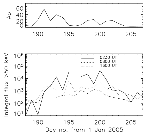
Figure 9. An example of the magnetic local time variation of the estimated integral >50 keV precipitation flux following a geomagnetic storm that started on 9 July 2005. The largest fluxes were measured in the midnight sector (0230 UT), with the morning sector showing slightly lower fluxes (0800 UT), and the afternoon sector fluxes the lowest (1600 UT). In all three time sectors, the integral fluxes remain elevated from the start of the storm on day 190 until day 205.
