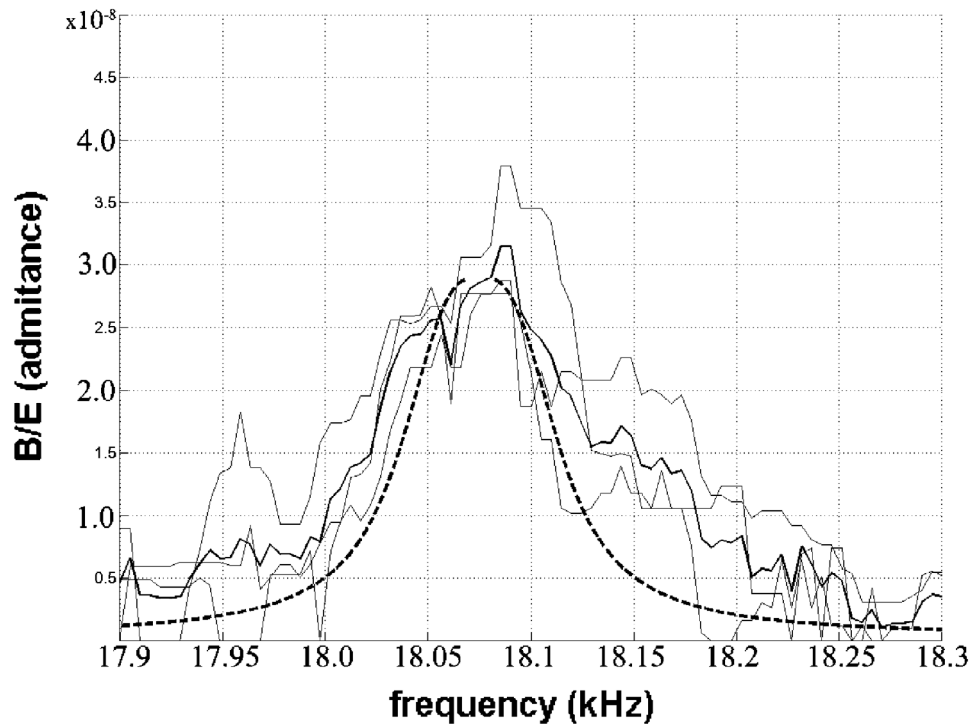
Figure 8. Comparison between the calculated admittance (a dotted curve; \omega_0/\omega_{He} = 2.5 , \omega/\omega_{He} = 0.02 ) and a set of experimental data curves of B/E .
