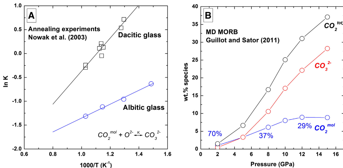
Fig. 1. A) Evolution of the equilibrium constant (K) for the interconversion reaction between CO 3 2- and CO 2 mol from annealing experiments of Nowak et al. (2003) on albite and dacitic compositions. B) CO 2 solubility (CO 2 tot ) and speciation (CO 2 mol and CO 3 2- groups) in MORB as a function of pressure (up to 15 GPa) derived from classical molecular dynamics simulations from Guillot and Sator (2011). Both studies imply the existence of a non-negligible abundance of CO 2 mol at high temperature in the melt.
