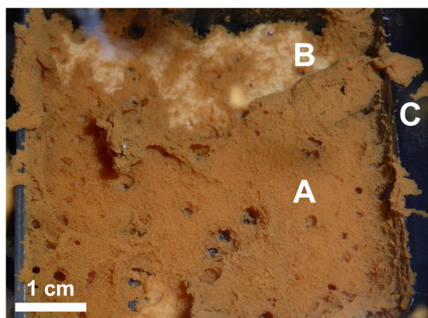
Fig. 10. Picture of a porous (>90%) mantle obtained after sublimation of an intra-mixture of 0.1% tholins and H 2 O ice particles, 70 μm in diameter. The sublimation lasted about 40 h at pressure <10 -5 mbar and a surface temperature of 200–220 K in the SCITEAS simulation chamber. A: porous mantle made of water-free tholins; B: bright fresh ice particles exposed to the surface after ejection of a large fragment of the mantle; C: fragments of mantle ejected from the surface of the sample and deposited onto the sample holder.
