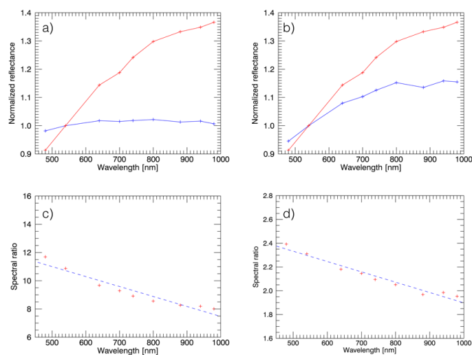
Fig. 11. a) and b) normalized reflectance spectra corresponding to different steps of a sublimation experiment using μm-sized H 2 O ice mixed with 5 wt.% basaltic airfall ash and 1 wt.% nanoparticle carbon as initial material. The red spectra in plots a) and b) are those of the final material at the end of the sublimation experiment. The blue spectrum in plot a) was acquired at the very beginning of the sublimation. The blue spectrum in plot b) was acquired about 10 h later. All spectra were normalized to their value of reflectance at 535.7 nm. c) and d) corresponding spectral ratios between the blue curves and red curves in plots a) and b) , respectively (crosses) and linear fit through these points (dashed lines).
